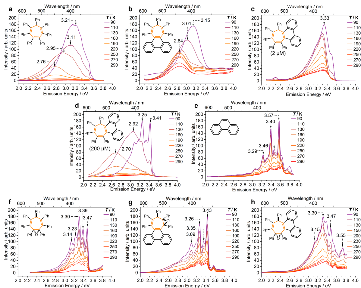
Figure 2. VT steady-state photoluminescence spectra of 2-MeTHF solutions of (a) Ph 7 C 7 H , excitation energy E_{\text{ex}} = 3.95 eV, concentration c = 2 \mu\text{M} , (b) sym-phenPh 5 C 7 H , E_{\text{ex}} = 4.13 eV, c = 2 \mu\text{M} , (c) asym-phenPh 5 C 7 H , E_{\text{ex}} = 3.95 eV, c = 2 \mu\text{M} , (d) asym-phenPh 5 C 7 H , E_{\text{ex}} = 3.95 eV, c = 200 \mu\text{M} , (e) phenanthrene, E_{\text{ex}} = 4.13 eV, c = 2 \mu\text{M} , (f) Ph 7 C 7 H-O , E_{\text{ex}} = 4.35 eV, c = 2 \mu\text{M} , (g) sym-phenPh 5 C 7 H-O , E_{\text{ex}} = 3.95 eV, c = 2 \mu\text{M} , and (h) asym-phenPh 5 C 7 H-O , E_{\text{ex}} = 3.95 eV, c = 2 \mu\text{M} .
