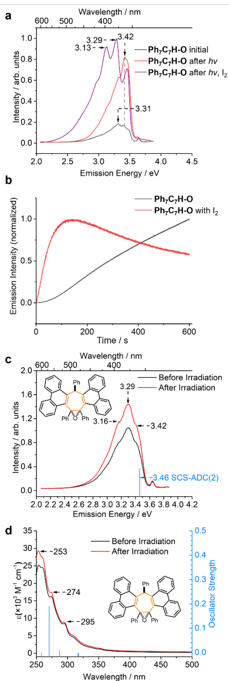
Figure 3. Steady-state photoluminescence spectra of 2-MeTHF solutions of \text{Ph}_7\text{C}_7\text{H-O} , ( E_{\text{ex}} = 4.35 \text{ eV} , c = 2 \mu\text{M} ) (a) before and after irradiation with 4.0 eV light for 10 min with and without \text{I}_2 ; (b) the change in the emission intensity at 3.30 eV over time, with and without \text{I}_2 ; (c) emission (2-MeTHF, c = 2 \mu\text{M} ) and (d) absorption (MeCN, c = 20 \mu\text{M} ) spectra of sym-phen 2 Ph 3 C 7 H-O before and after irradiation with 4.0 eV light for 10 min. Theoretical emission (vertical transition from the \text{S}_1 geometry) and absorption (five lowest vertical transitions from the \text{S}_0 geometry) transitions shown in panels c and d were obtained at the SCS-ADC(2)/TZVP//SCS-ADC(2)/SVP and SCS-ADC(2)/TZVP//SCS-MP2 levels of theory, respectively.
