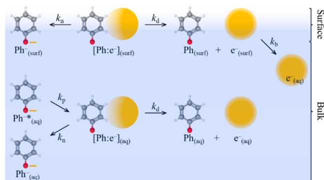
Figure 2. Schematic of kinetic models following photo-oxidation from phenolate at the water/air surface (surf) and in aqueous solution (aq). Phenolate, \text{Ph}^- , is photoexcited, \text{Ph}^* , and forms a contact pair [\text{Ph}:e^-] with a rate coefficient k_p . [\text{Ph}:e^-] can either dissociate to the phenoxyl radical, \text{Ph} , and e^- , with a rate coefficient k_d or undergo geminate recombination to reform \text{Ph}^- with a rate coefficient k_n . The e^-_{(surf)} can additionally diffuse into the bulk with a rate coefficient k_b . At the surface, k_p has been omitted for clarity.
