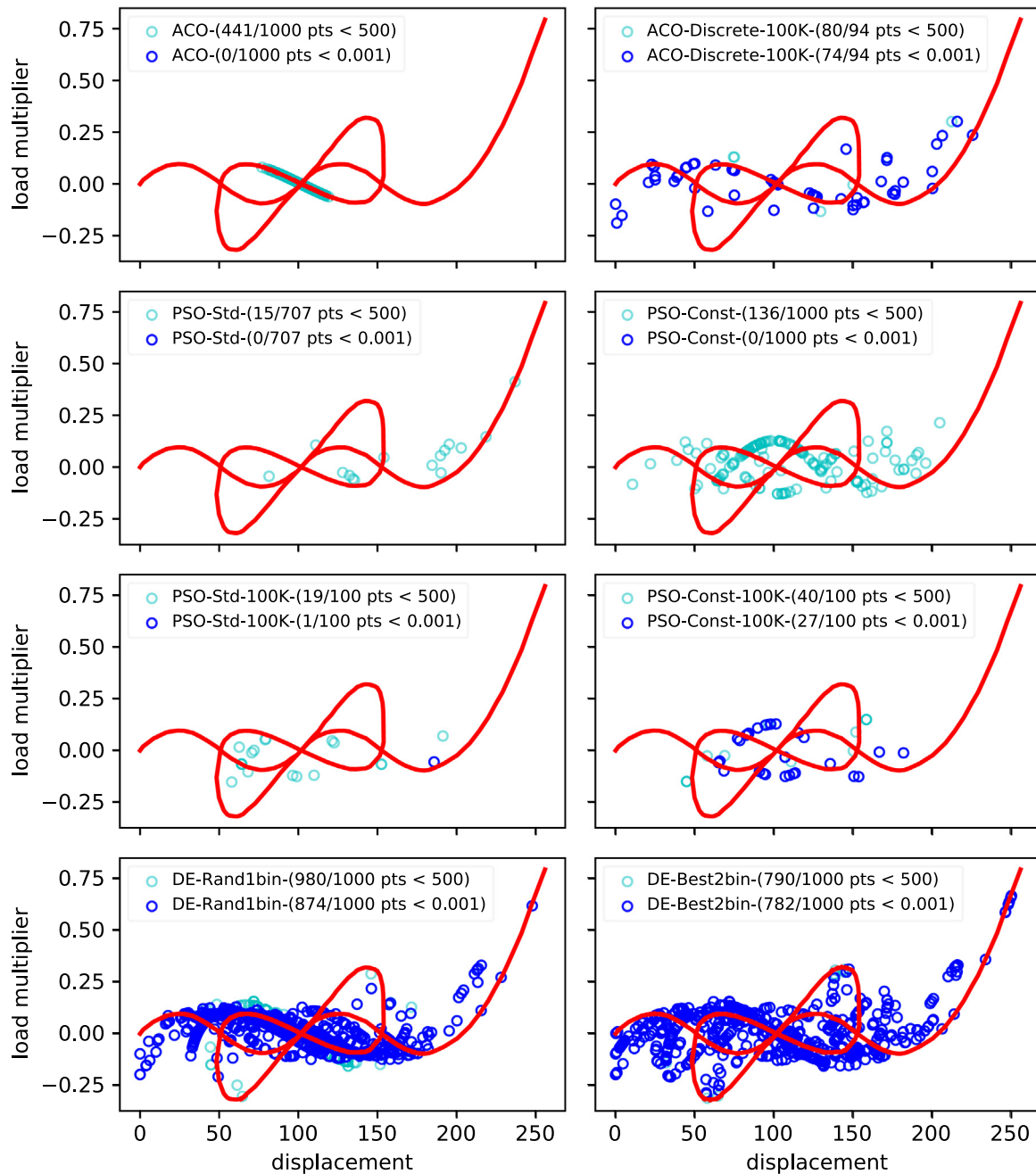
Fig. 12. Quality of solutions (in blue solutions with a precision of 0.001 as their equilibrium value and solution in cyan are with precision 500) produced by optimization algorithms over 10 000 generations and 100 000 generations for ACO-Discrete and PSO-100K versions. Arc-length method based equilibrium path is shown in red. From top-left to bottom-right algorithms are ACO, ACO (with a discrete domain of control points over 100 000 generations), PSO-Std, PSO-Const, PSO-Std with 100 000 generations, PSO-Const with 100 000 generations, DE/rand/1/bin, and DE/best/2/bin.
