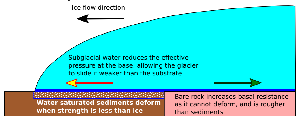
Fig. 1. Schematic of the components of the new basal conditions model. (a) Overview of ice sheet hydrology. (b) Overview of impact on sliding.
