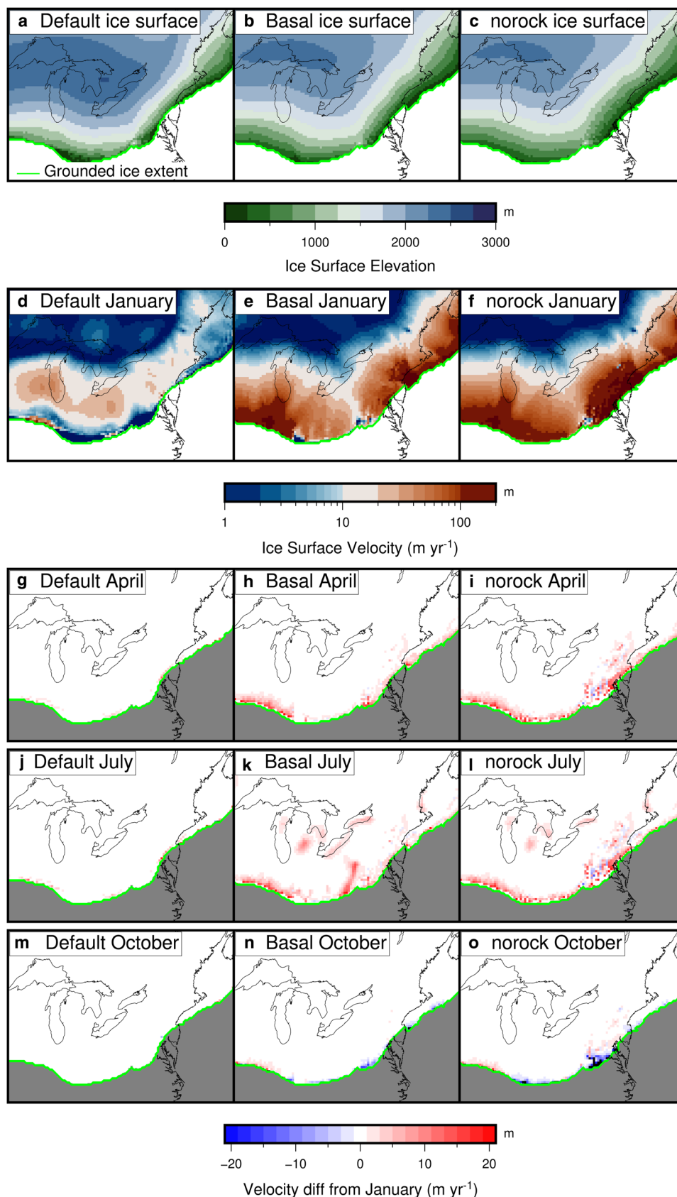
Fig. 10. Comparison of ice surface elevation (a–c) and ice surface velocity in January (d–f) and the difference in velocity compared to January (g–o) for the three simulations for the southwestern Laurentide Ice Sheet at 20 000 yr BP.
