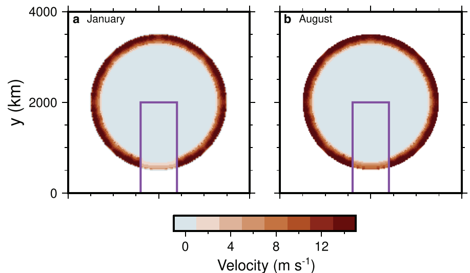
Fig. 5. Comparison of ice sheet surface velocity between the winter and summer for the simulation shown on Figure 3 at 25 000 years. The purple box shows the region that has S_f = 50\% sediment cover. (a) In the winter, the velocity in partially sediment cover is near zero, while the margin regions with continuous cover continue to flow. (b) In the summer, the velocity in partially covered areas increases as a result of the input of water.
