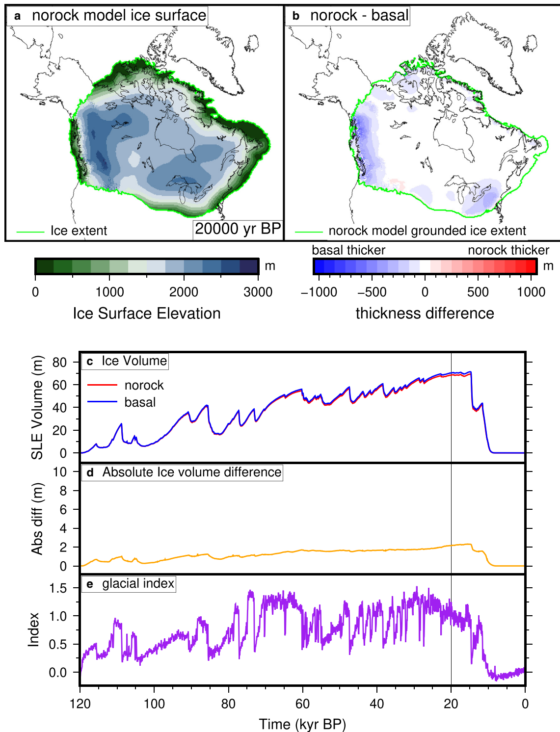
Fig. 9. Same as Figure 7, but comparing a simulation with S_f=100\% sediment cover (norock) and with spatially variable sediment cover (basal). (a) The ice surface elevation of the norock simulation at 20 000 yr BP. (b) The difference between the basal and norock grounded ice thickness at 20 000 yr BP. (c) Ice volume evolution of the simulations. (d) Absolute ice volume difference (i.e. the absolute value of panel (b)) between the simulations. (e) Glacial index used in the simulations, based on the Greenland ice core records (Andersen, 2004).
