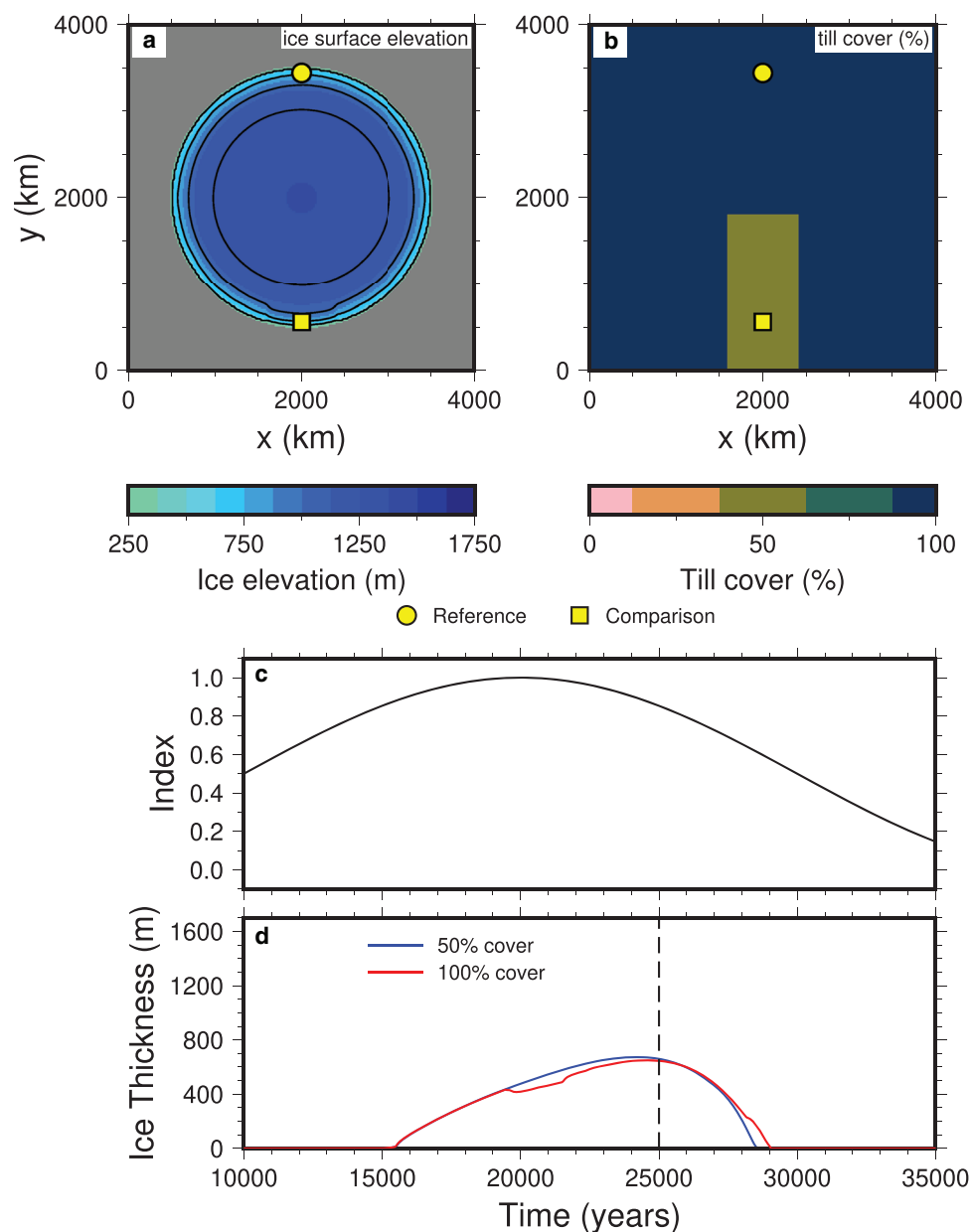
Fig. 3. Experiment with a strip of S_f=50\% sediment cover, with \gamma_{rc}=2^\circ for areas with bare rock, and \gamma_{sc}=1^\circ for areas covered in sediment. For sediment deformation, \phi_{sed}=20^\circ . The percentage of surface meltwater reaching the base is 80%. (a) Ice surface elevation at 25 000 years. (b) Sediment (till) cover fraction, showing the strip with reduced cover. Also shown are the locations that are used to compare the velocity and sliding properties. (c) Index used to linearly interpolate the climate variables, where 0 is warm conditions, while 1 is glacial conditions. (d) Ice thickness evolution at those two locations, showing a greater thickness in the partially covered strip, as the velocity is less.
