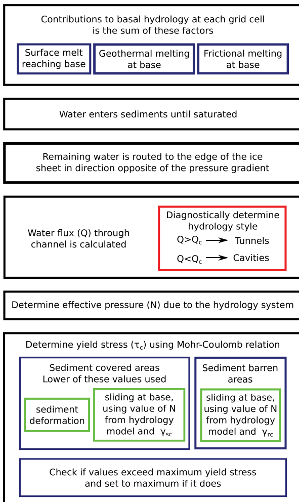
Fig. 2. Diagram showing the workflow of the model.
