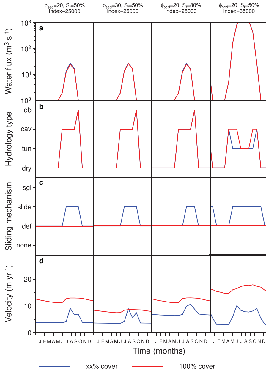
Fig. 4. Basal conditions and velocity time series for the locations shown in Figure 3 at about 25 000 years with S_f values of 50% or 80% (blue lines) and 100% (red lines) and \phi_{sed} values of 20° and 30° and glacial index set to 25 000 years or 35 000 years. (a) Volume water flux, primarily from meltwater from the surface being transferred to the base. (b) Type of water routing at the base of the ice sheet that determines the effective pressure. ob - overburden, cav - cavities, tun - tunnels/channels, dry - no water in the system. (c) Sliding law method used by PISM. sgl - slippery grounding lines, slide - modified sliding law that takes into account both sediment deformation and sliding at the ice-bed interface, sed - sediment deformation only model (PISM default), none - no sliding (i.e. no ice is present). (d) Surface velocity magnitude.
