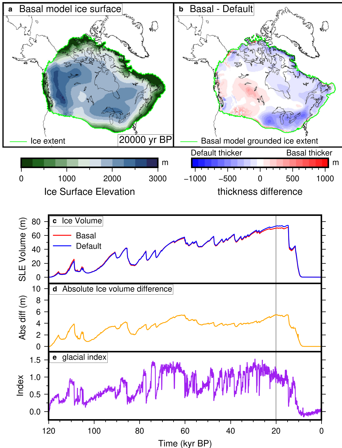
Fig. 7. Results of the glacial cycle simulation, comparing the default and basal simulations. (a) The ice surface elevation of the basal simulation at 20 000 yr BP. (b) The difference between the basal and default grounded ice thickness at 20 000 yr BP. (c) Ice volume evolution of the simulations. (d) Absolute ice volume difference (i.e. the absolute value of panel (b)) between the simulations. (e) Glacial index used in the simulations, based on the Greenland ice core records (Andersen, 2004).
