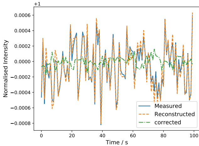
Figure 17. An example simulated light curve for the 4LGSF on the VLT. The measured normalised intensity, tomographically reconstructed normalised intensity and corrected intensity are plotted.
