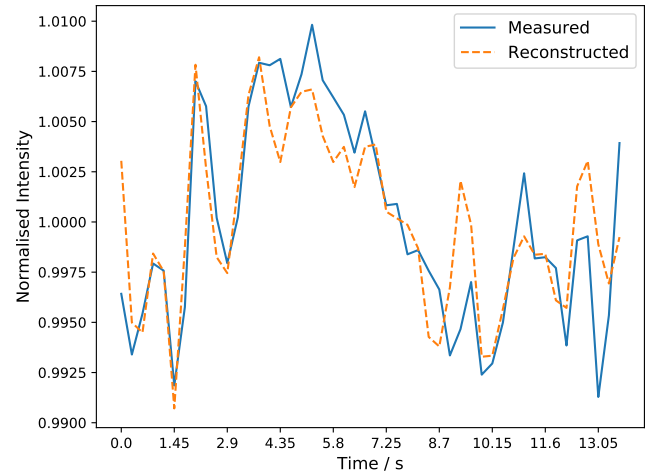
Figure 10. The measured normalised intensity and the normalised tomographically reconstructed intensity for the best performing 0.1s data packet. The intensity was temporally binned by a factor of 2.
