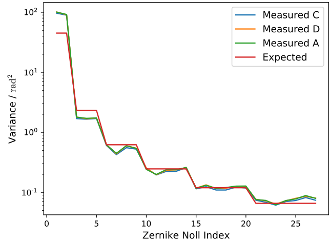
Figure 6. The measured Zernike mode variance for Theta-1 Orionis C, D and A. The expected variance for r_0 = 0.16\text{m} is also plotted.
