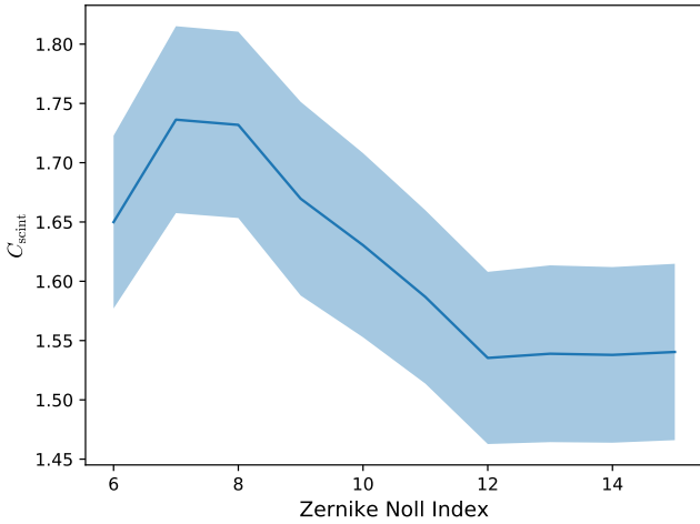
Figure 7. The average measured scintillation correction factor as a function of the Noll index for the 0.1s data packets. A peak around 8 modes suggest that only low orders are required for the scintillation correction.
