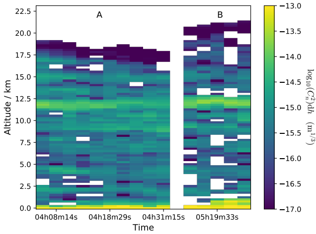
Figure 8. The turbulence profiles measured over 1.5 hours of the night of the 19th of September. The observations are split into observing period A and B with a gap between the observations plotted. A strong turbulent layer is seen at the ground and at 12km.
