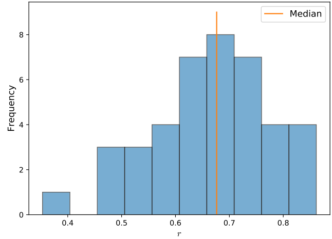
Figure 12. A histogram of the measured correlation coefficient between the measured intensity and tomographically reconstructed intensity. The median of the measured correlations is also plotted.
