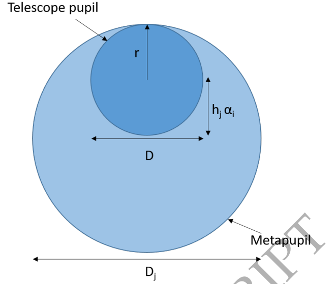
Figure 2. A schematic showing the de-centered part of the meta-pupil at altitude h_j seen by the WFS in direction \alpha_i .
