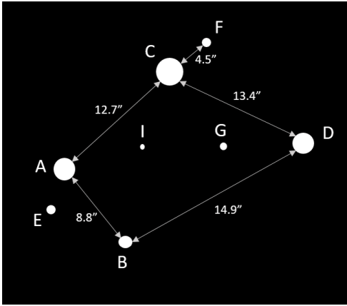
Figure 3. A schematic showing the Orion Trapezium Cluster. Each label defines the name of the star, with Theta-1 Orionis A given by label A, Theta-1 Orionis B given by label B and Theta-1 Orionis C given by label C etc. The stars used to perform the tomography are Orionis A, C and D.
