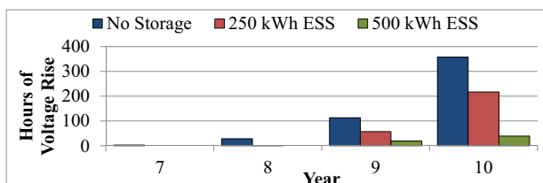
Figure 4: Hours of voltage rise per annum (scenario 2)
