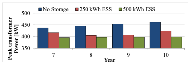
Figure 3: Peak power through transformer (scenario 1)
