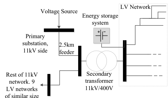
Figure 1: Overview of network under study
