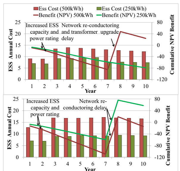
Figure 5: NPV of DNO benefits and ESS cost over investment period: scenario 1 (top), scenario 2 (bottom)
