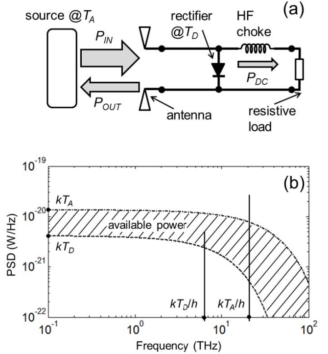
Fig. 1. (a) Rectenna circuit model. The input power P_{IN} is black-body radiation emitted by the source and collected by the antenna, while P_{OUT} is the power lost by the rectifier at a finite temperature. (b) Power spectral density (PSD) of P_{IN} and P_{OUT} at the antenna feedpoint. The hatched area is the maximum available power available for conversion. T_A = 973 K and T_D = 296 K, the quantum cutoff kT/h is shown in the graph.
