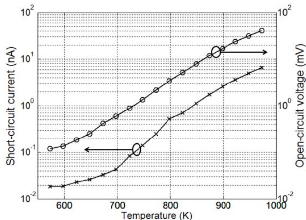
Fig. 2. Rectenna short-circuit current I_{SC} and open-circuit voltage V_{OC} as a function of the source temperature T_A . The rectenna temperature T_D was maintained at a constant temperature of approximately 296 K.
