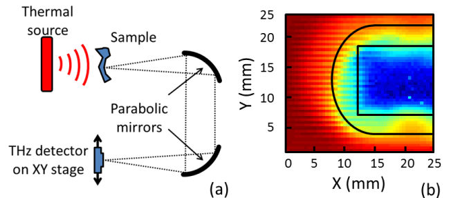
Fig. 1. (a) Diagram of the broadband THz imaging system. The thermal radiation from the black-body source is transmitted through the sample and focused on the self-switching nanodiode detector. (b) The image of a USB memory stick. THz radiation penetrates through the plastic case (yellow area), but is completely stopped by the metal connector (blue area).
