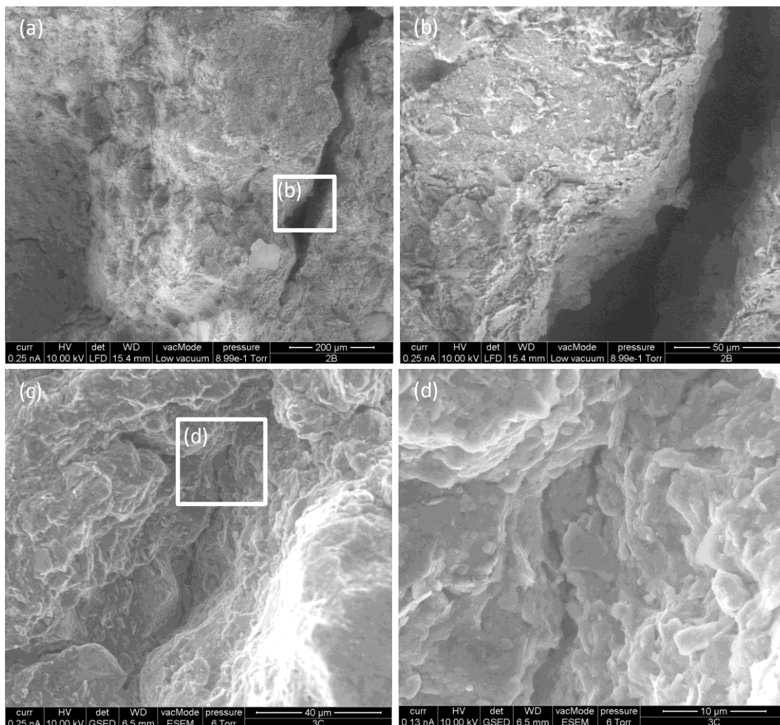
Figure 12. E-SEM images taken at two sites (a) site 1 after 90 min at 10% RH and showing the position of (b) desiccated clay particles and fracture wall under higher magnification, (c) site of reduced crack aperture following re-wetting and the position of (d) hydrated particles under higher magnification (after Hen-Jones et al. 2015).
