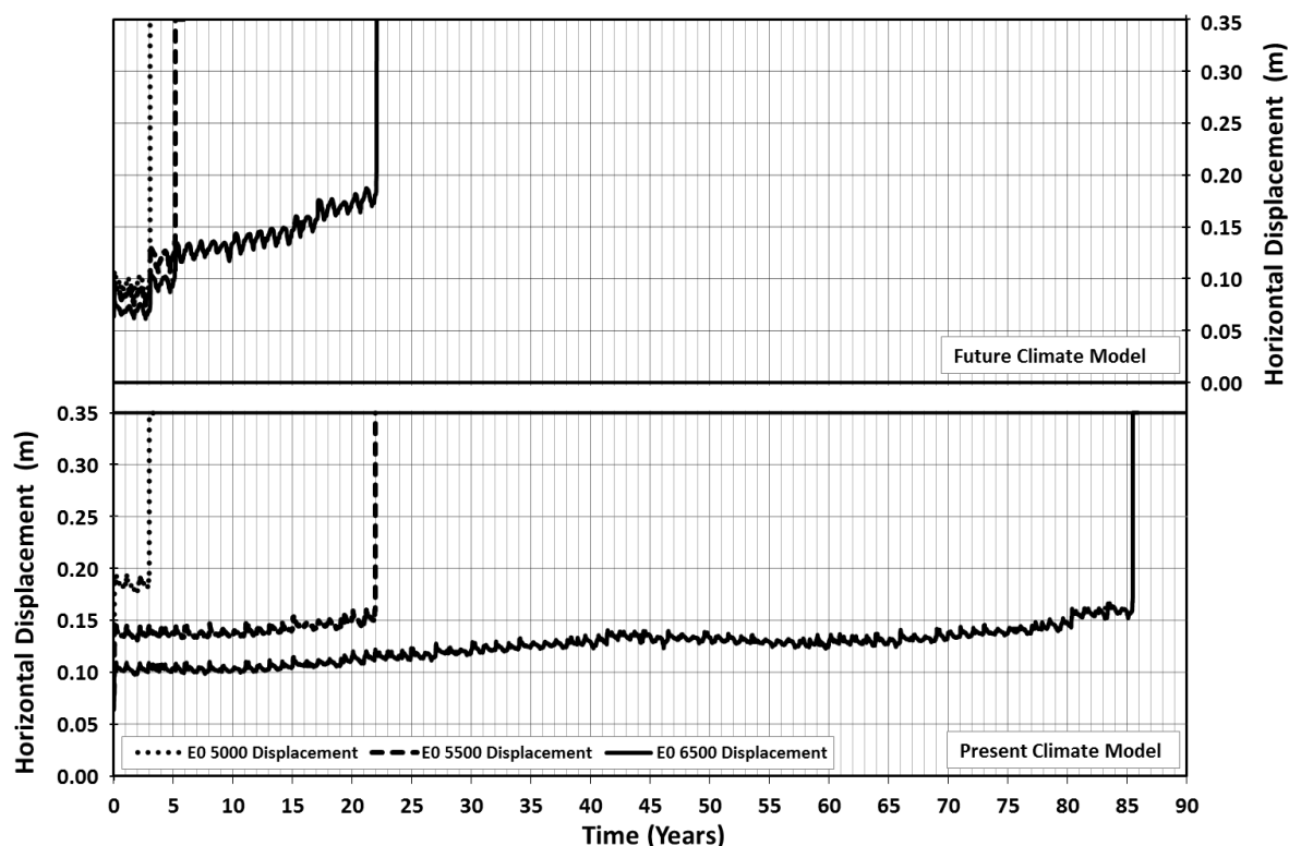
Figure 14. Effect of pre-failure stiffness on cut-slope stability due to imposed present and future climates.
