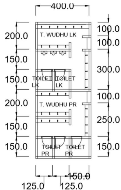
Gambar 4.15. existing toilet masjid At-taqwa
