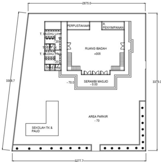
Gambar 4.3. denah existing area parkir masjid At-taqwa
