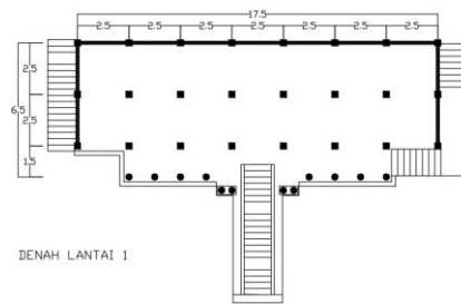
Gambar 2 Denah Lantai 1 Masjid Jami' Sunan Abinawa
