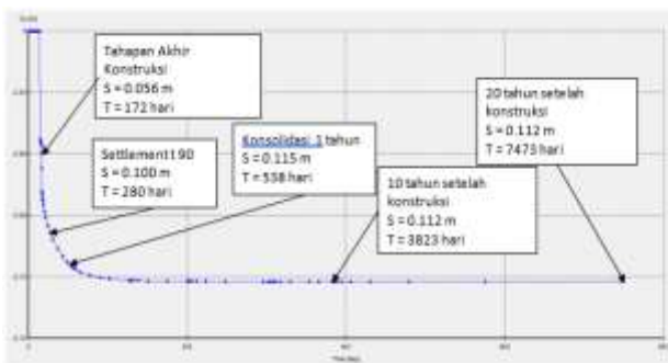
Gambar 9. Kurva Settlement
