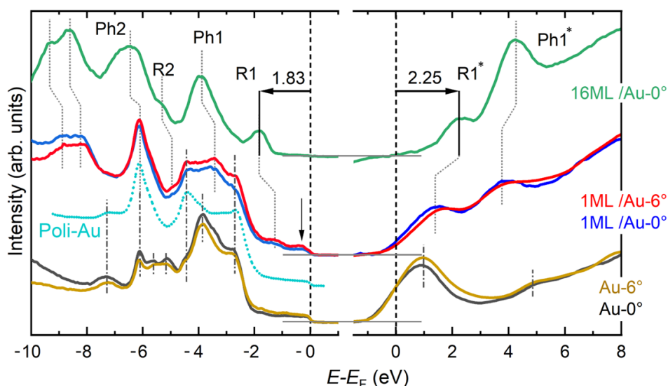
Figure 3: Normal emission UPS and normal incidence IPES spectra for 16 ML CoTPP, 1 ML CoTPP and the substrates. Both the flat and the vicinal Au sample spectra are shown. The spectrum of polycrystalline Au, shown in turquoise, is adapted from Ref. [36]. The spectroscopic contributions from phenyls (Ph) and the tetrapyrrole ring (R) of the porphyrin molecules are labelled in the image as per Ref. [47].
