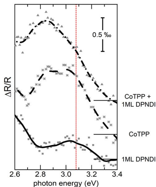
Figure 7: From bottom to top: RAS spectra acquired on 1ML DPNDI, 1 ML CoTPP and the DPNDI:CoTPP axial complex, all grown on vicinal Au(001)-6°. The red line at a photon energy of 3.1 eV marks the position of peak DPNDI optical absorption.
