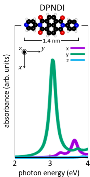
Figure 6: Calculated absorbance for the free DPNDI molecule.
