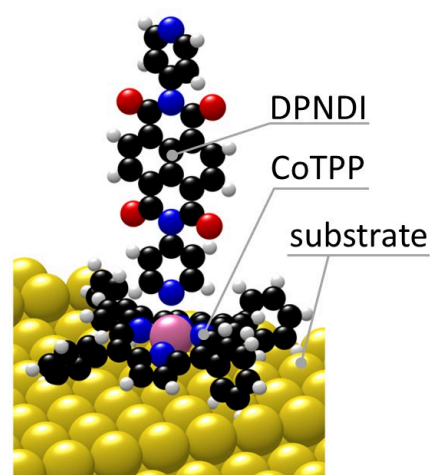
Figure 1: Schematics of the axially coordinated DPNDI:CoTPP complex. Color code: yellow = gold, pink = cobalt, black = carbon, blue = Nitrogen, red = oxygen, white = hydrogen.
