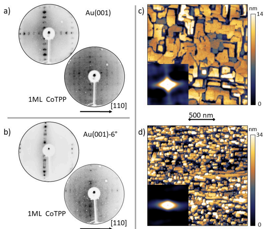
Figure 2: LEED patterns acquired at 55 eV for the bare substrate and 1 ML of CoTPP on a) flat Au(001) and b) vicinal Au(001)-6°. AFM images acquired for 16 ML of CoTPP on c) flat Au(001) and d) vicinal Au(001)-6°. Insets (c, d): 2D autocorrelation function of the AFM images. The crystallographic directions are the same for both LEED and AFM.
