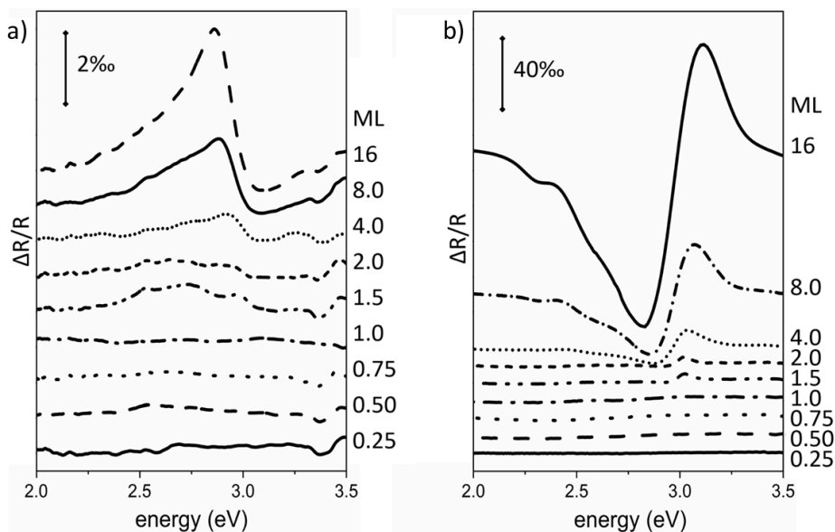
Figure 4: Incremental RAS spectra acquired during the growth of CoTPP on a) flat Au(001) and b) vicinal Au(001)-6°.
