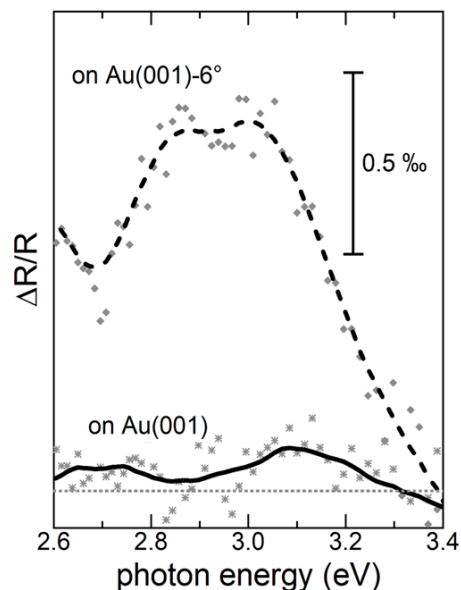
Figure 5: RAS signals for 1 ML CoTPP on Au(001) and Au(001)-6°.
