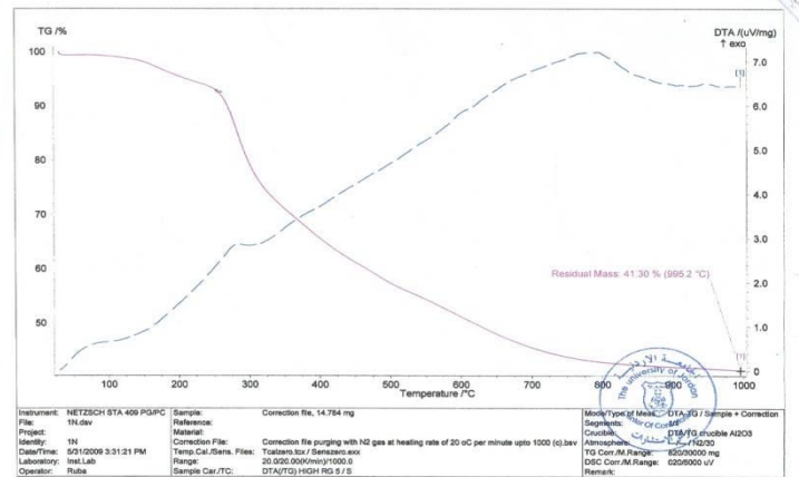
Fig (18) Curing Thermogram of Compound (8)
