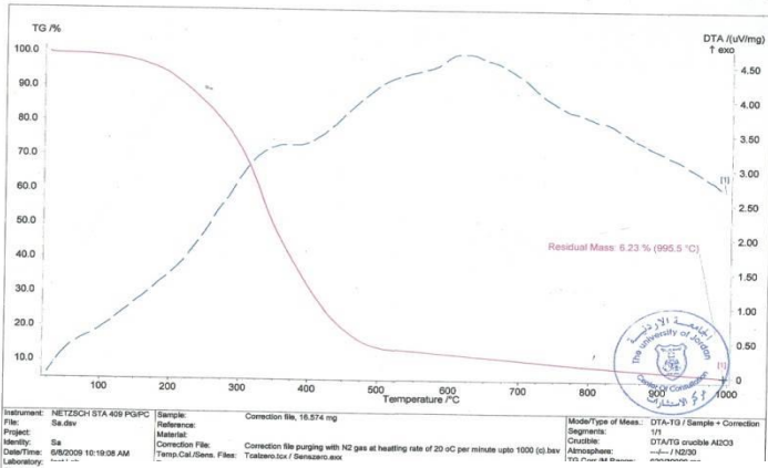
Fig (15) Curing Thermogram of Compound (4)
