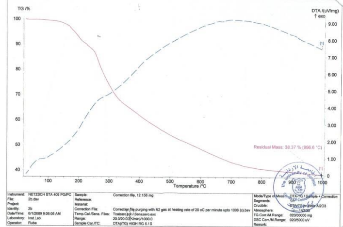
Fig (18) Curing Thermogram of Compound (8)
