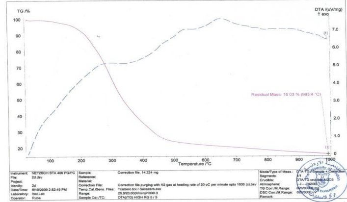
Fig (16) Curing Thermogram of Compound (5)
