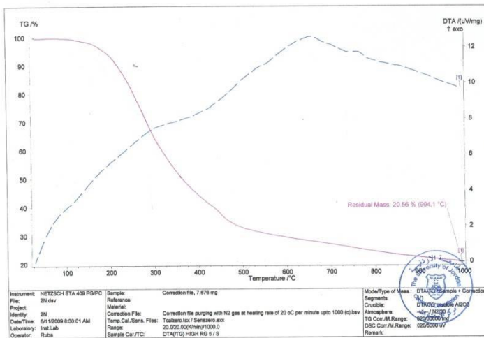
Fig (17) Curing Thermogram of Compound (6)
