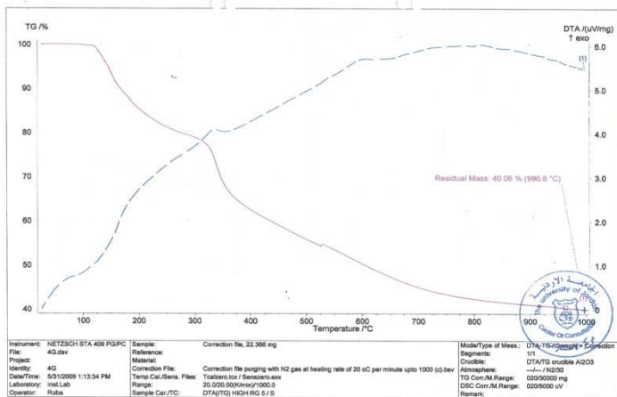
Fig (19) Curing Thermogram of Compound (9)
