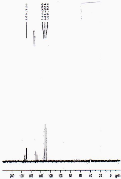
Fig (13) 13 CNMR Spectrum of Compound (3)
