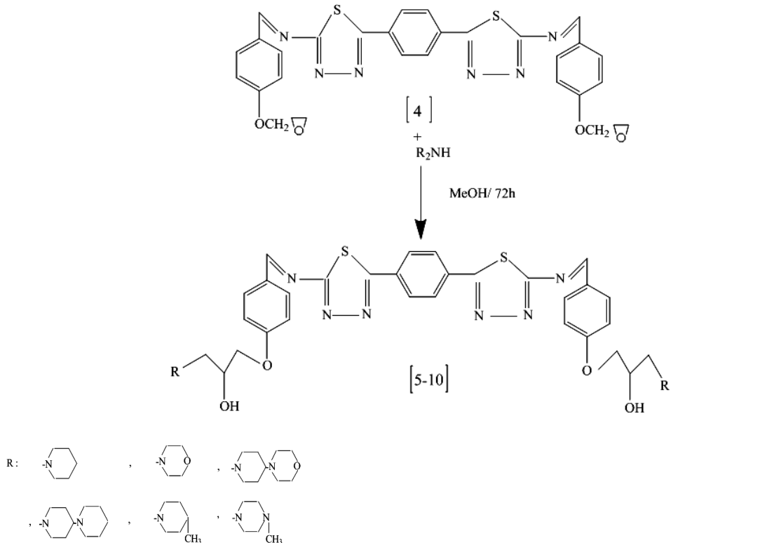
Scheme – 5 – Synthetic path ways for preparation of Compound (5-10)
