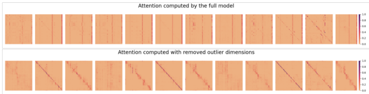
Figure 6: The self-attention patterns at the 10th layer of the full ‘bert-base-uncased’ pre-trained model vs the same model with removed LayerNorm outliers.
