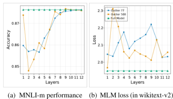
Figure 10: RoBERTa-base: effect of disabling outliers.
