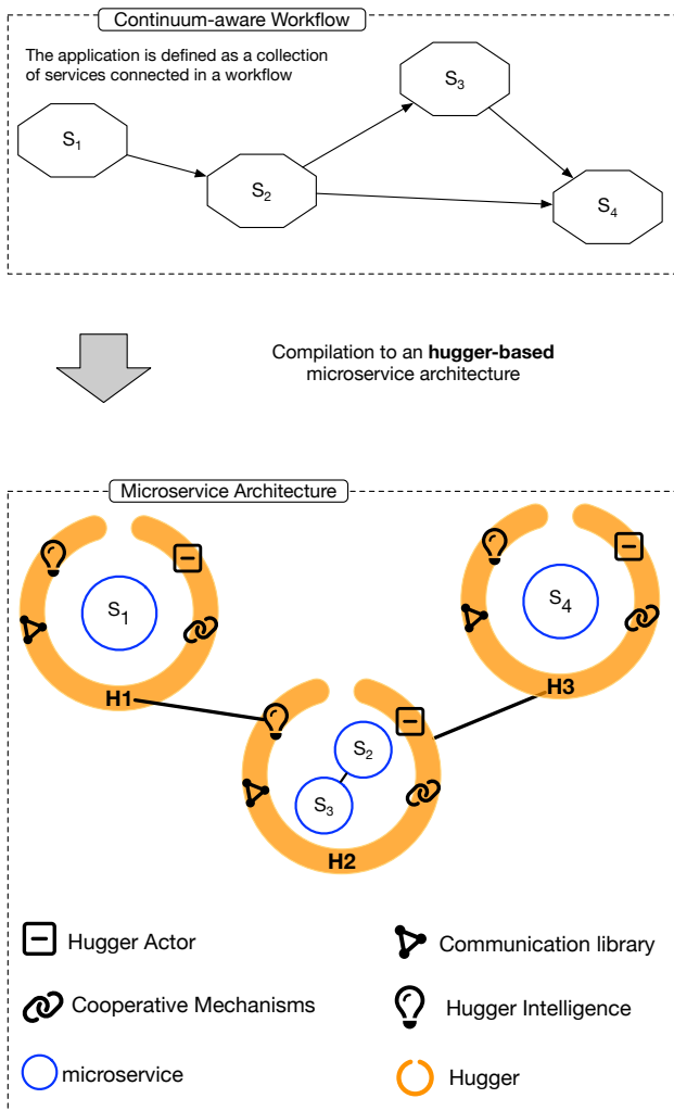
Fig. 1. From workflows to Huggers
