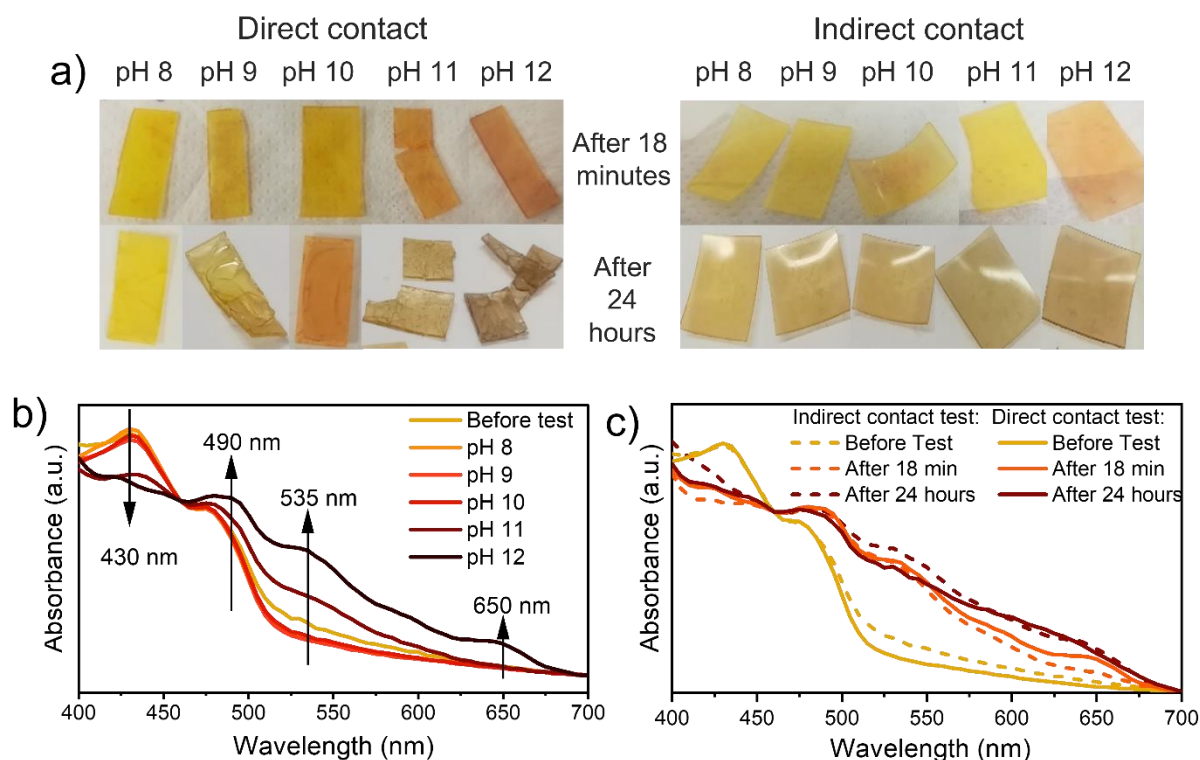
Figure 3. a) Pictures of P575_NDI-OH samples after 18 minutes or 24 hours of direct and indirect contact test with NH 3 /H 2 O solutions at different pH; b) visible absorption spectra of P575_NDI-OH samples tested for 18 minutes by direct contact with NH 3 /H 2 O solutions at different pH; c) comparison between the absorption spectra of P575_NDI-OH samples tested at pH 12 for 18 minutes and 24 hours by direct and indirect contact test.
