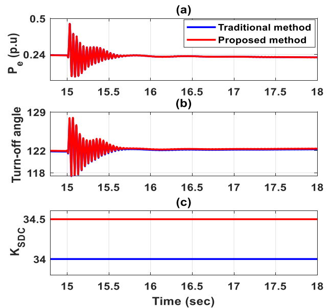
FIGURE 13. Electric power, turn-off angle, and K_{SDC} when K=70\% and V_w=7 m/s.
