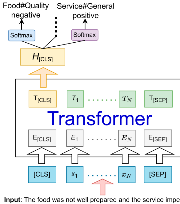
Figure 4. The overall architecture is based on the pre-trained transformer language models for the Category-Sentiment Classification task.
