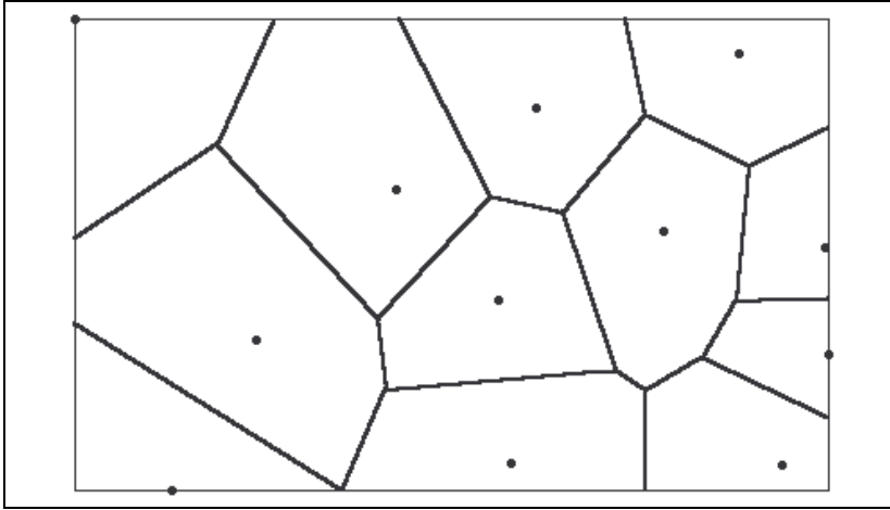
Fig. 2.2.3b: Division of the domain of the interpolation function.
