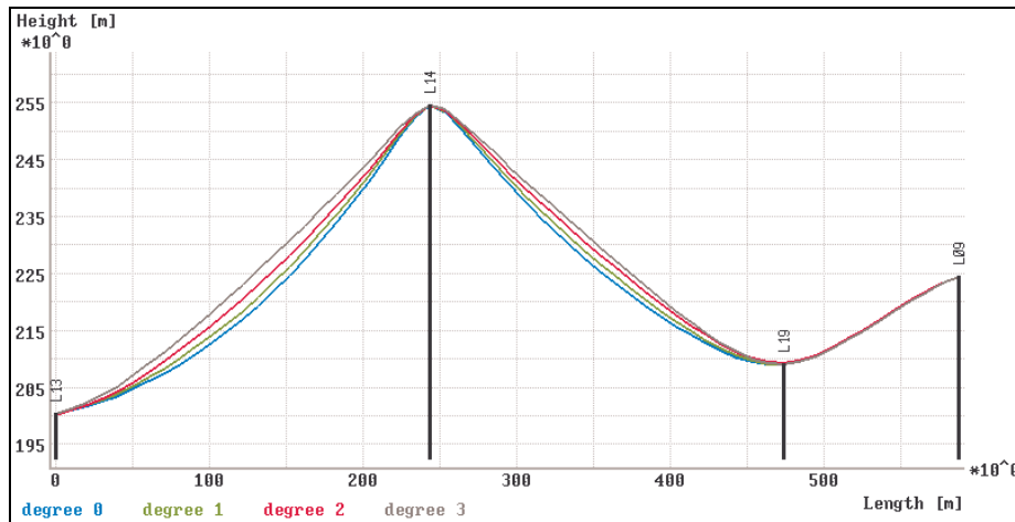
Fig. 3.4.2: Influence of the linear tensioning degree.
