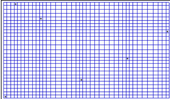
Fig. 4.2.9: Automatically created finite element model grid.
