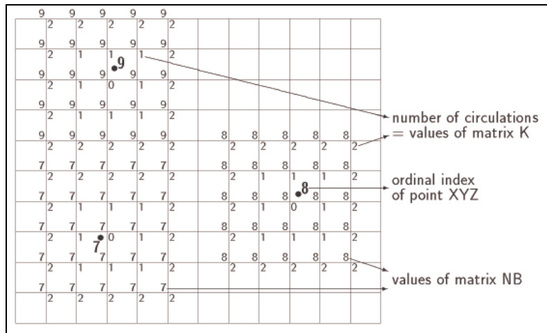
Fig. 2.2.3a: Computation of the matrices NB and K .
