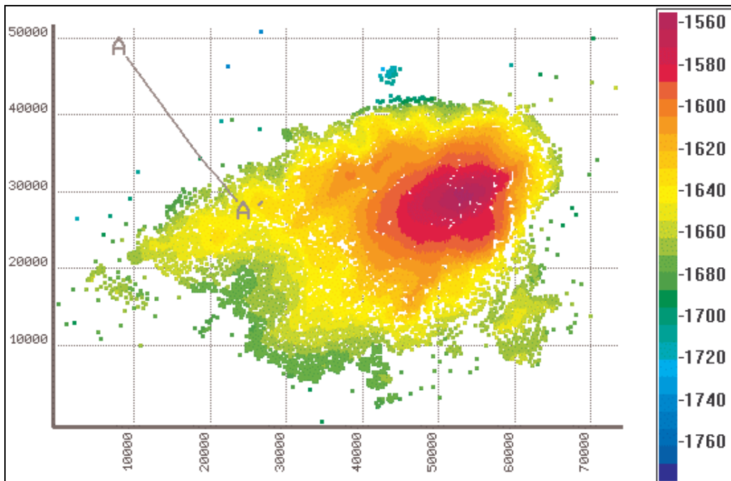
Fig. 2.4.3a: Distribution of points in the example SIBIR.
