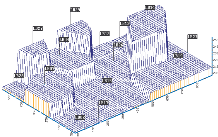
Fig. 2.2.4: Per partes constant interpolation.
