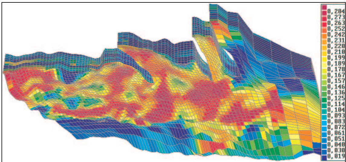
Fig. 5.8b: Porosity of a geological model.
