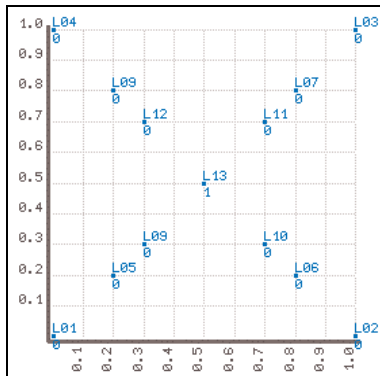
Fig. 2.4.1a: Distribution of points in the example OSCIL.
