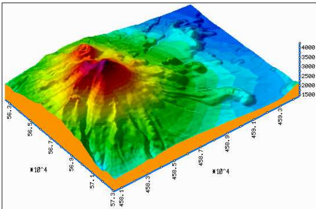
Fig. 5.7: Digital elevation model of mount Shasta in Northern California.
