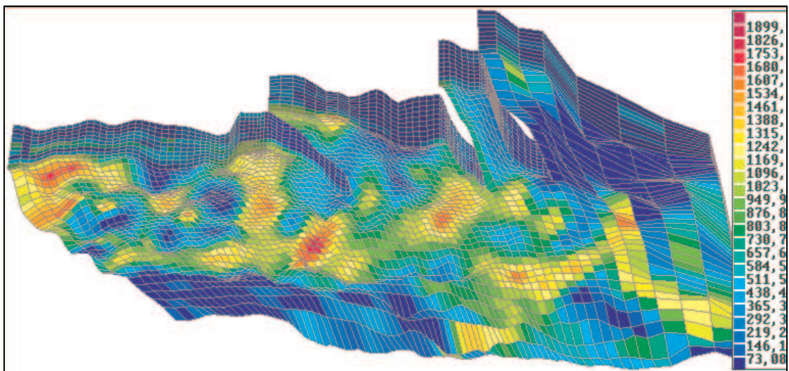
Fig. 5.8c: Permeability of a geological model.
