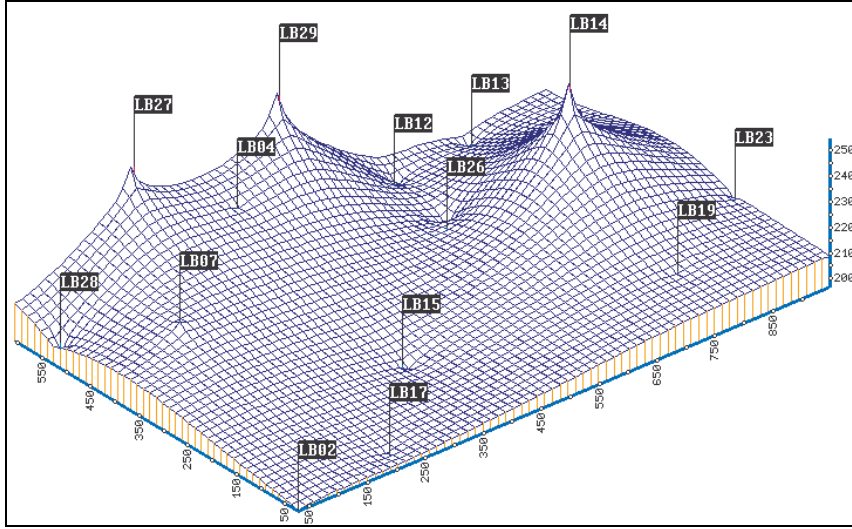
Fig. 2.2.5: Tensioning of the surface.
