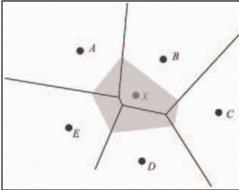
Fig. 1.2.2: New Voronoi cell and areas for computation of neighbour point weights.
