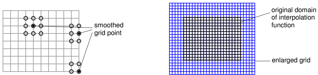
Fig. 3.4.3a: Nodes included in smoothing
