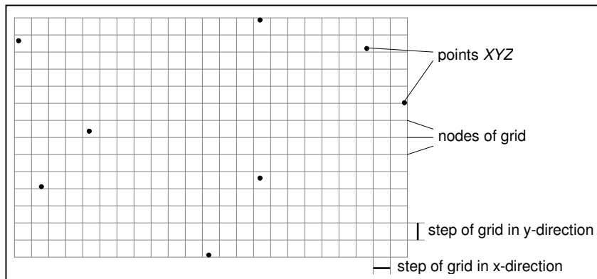
Figure 2.1: Regular rectangular grid for defining the interpolation function.
