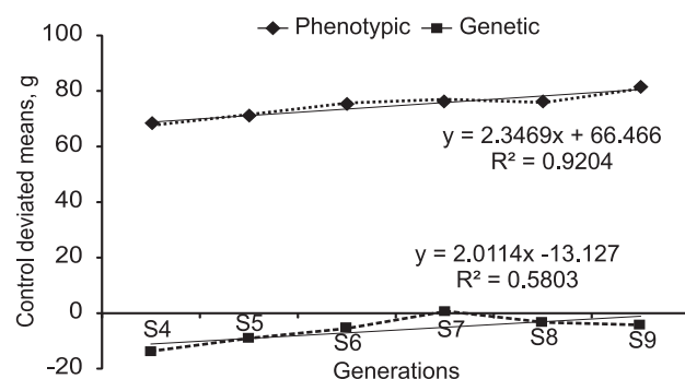
Fig. 1. Direct genetic and phenotypic response for primary trait shank length in PD-1 line.
