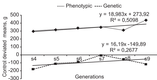
Fig. 3. Correlated responses (genetic and phenotypic) for 4-week-body weight in PD-1 line.
