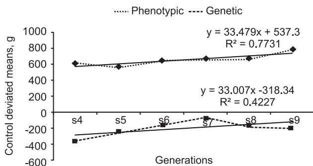
Fig. 4. Correlated responses (genetic and phenotypic) for 6-week-body weight in PD-1 line.
