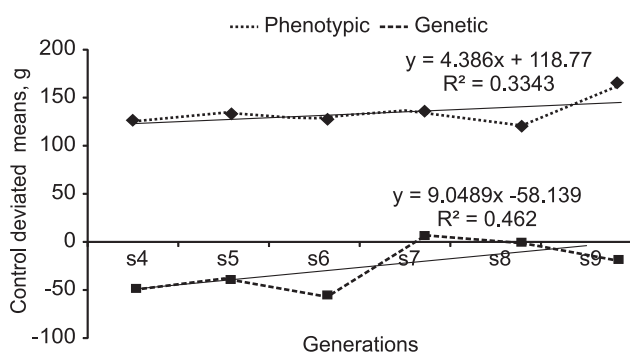
Fig. 2. Correlated responses (genetic and phenotypic) for second week body weight in PD-1 line.
