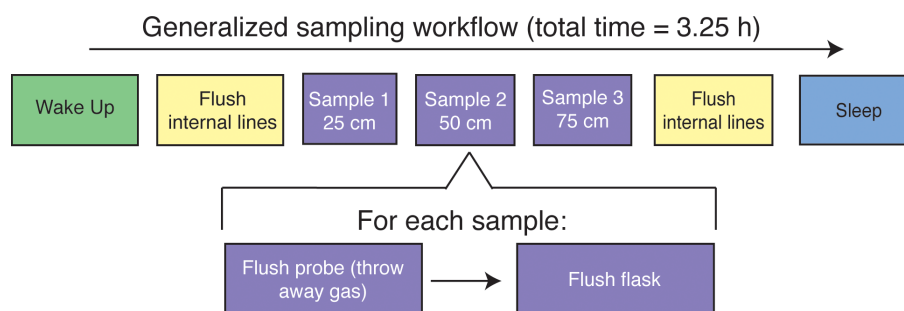
Figure 2. Flow chart of the instrument schedule used for sampling during all field experiments.
