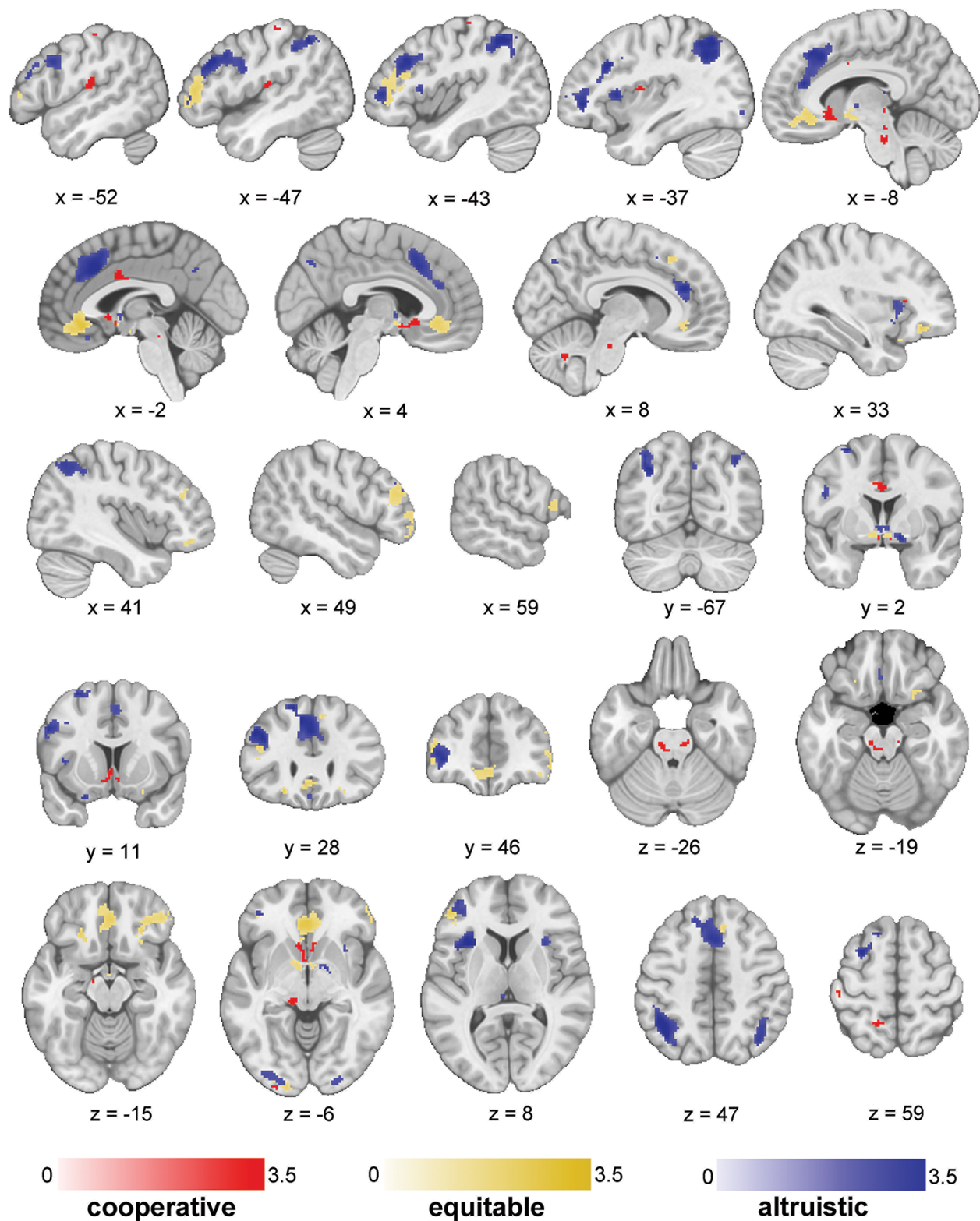
Fig. 3. Thresholded results from meta-analyses.
