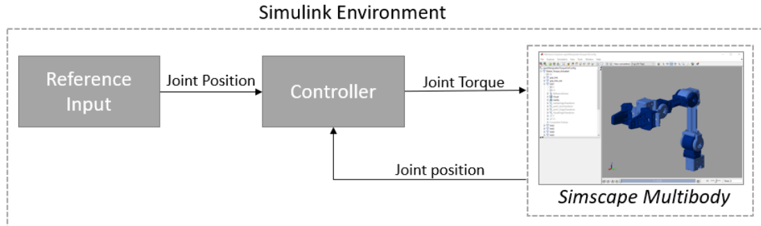
Figure 2.2: Controller scheme using Simscape Multibody environment
