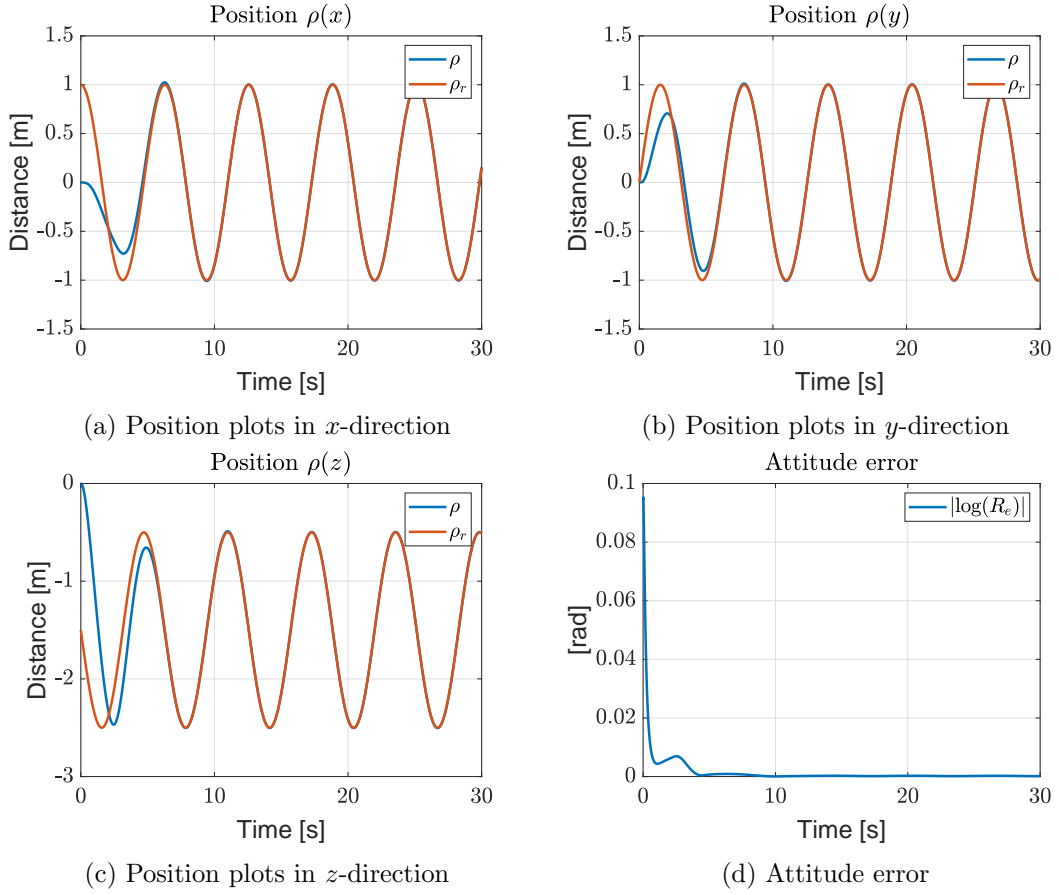
Figure 3.3: Simulation results using the model (3.1), the controller as described in section 3.3 and the initial conditions (3.32).
