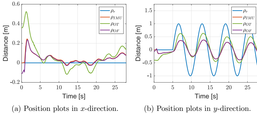
Figure 5.7: Experimental results where the IMU, Optitrack and optical flow data are equalized after 6 seconds. It shows that the IMU and optical flow data are nearly identical.
