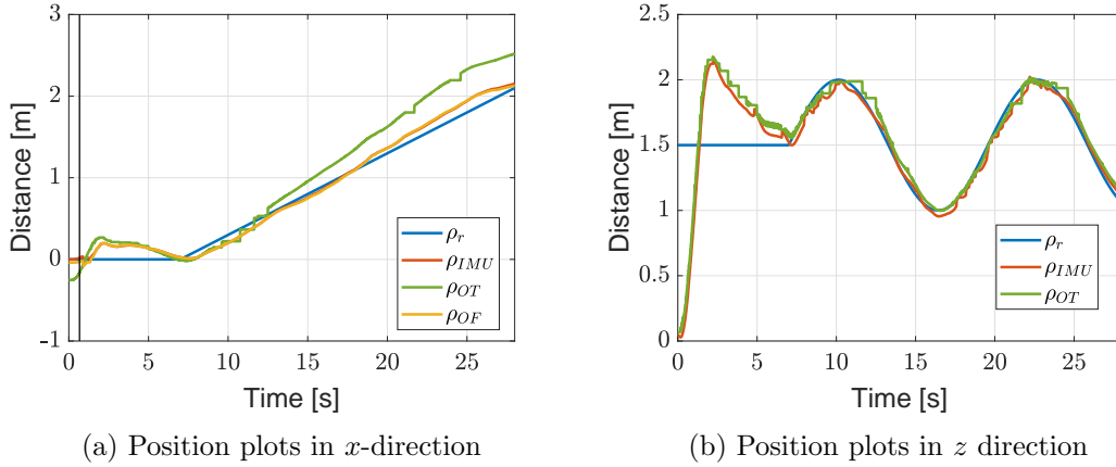
Figure C.2: Experimental results of a trajectory with constant horizontal speed and a varying height.
