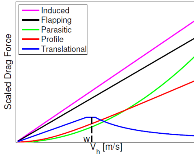
Figure 3.2: Impression of the magnitude of the described types of drag with respect to velocity of the drone [2]
