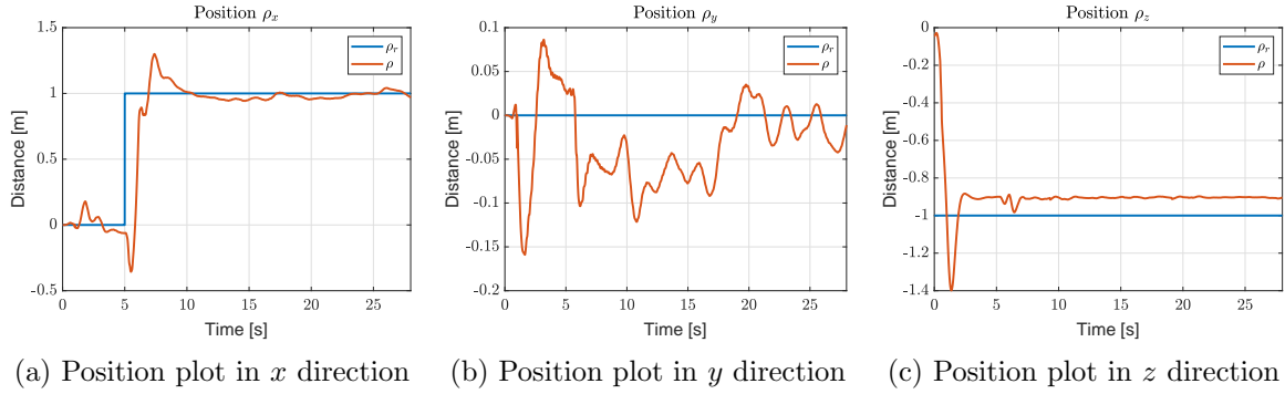
Figure 4.3: Experimental results of a step function using the default estimator and controller of the support package.
