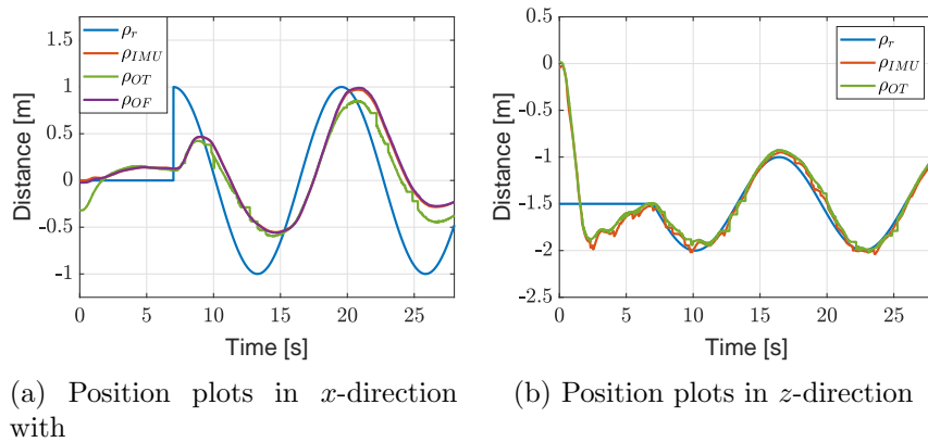
Figure C.4: Position plots for the circular trajectory in x and z direction for the original optical flow factor.
