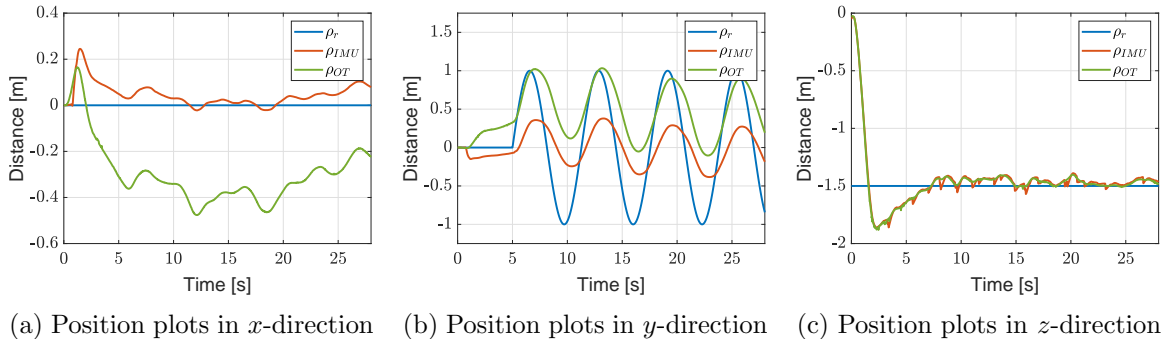
Figure 5.4: Experimental results with the reference signals in blue \rho_r , the estimated values by the default estimator \rho_{IMU} in red and the Optitrack values \rho_{OT} in green.
