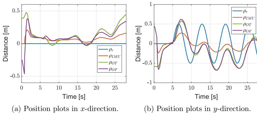
Figure 5.9: Experimental results of a trajectory at 2.5m altitude. This required a higher multiplication factor for the optical flow to acquire a signal similar to the Optitrack measurement.
