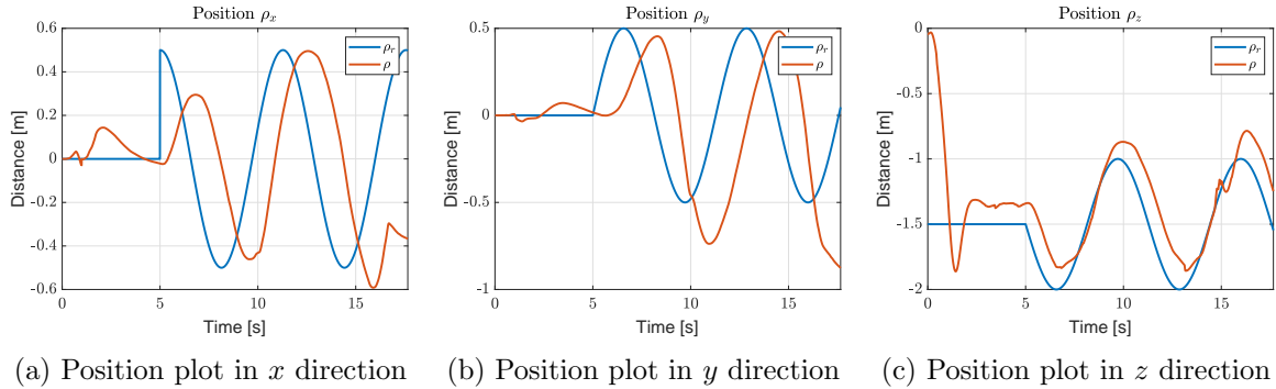
Figure 4.4: Experimental results with a circular reference trajectory using the default estimator and controller of the support package. The experiment has been terminated early because the Mambo has flown into its surroundings.
