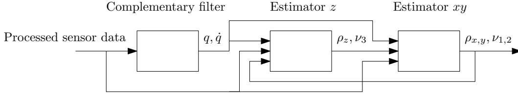
Figure 5.1: Schematic overview of the state estimation on the Mambo
