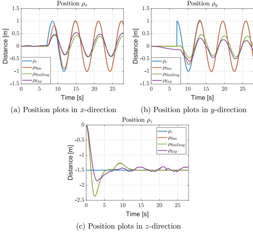
Figure 6.4: Experimental and simulation results of a circular trajectory with and without the drag included in the model, with k_c = 0.22 .
