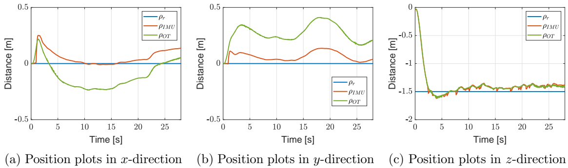
Figure 5.3: Experimental results with the reference signals in blue \rho_r , the estimated values by the default estimator \rho_{IMU} in red and the Optitrack values \rho_{OT} in green.
