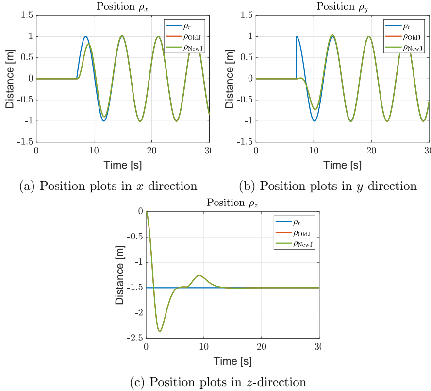
Figure 6.3: Simulation results of a circular trajectory with both the old and the new inertia. The red (old inertia) line is nearly identical to the green (new inertia) line.
