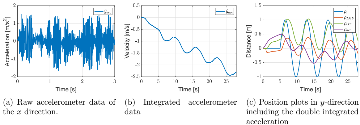
Figure 5.5: Accelerometer data and the corresponding velocity and position after calibration and integration.
