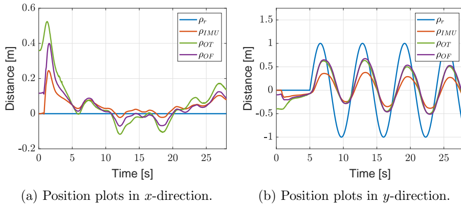
Figure 5.8: Experimental results with the optical flow data multiplied by a constant. Now the integrated optical flow is almost identical with the Optitrack measurement.
