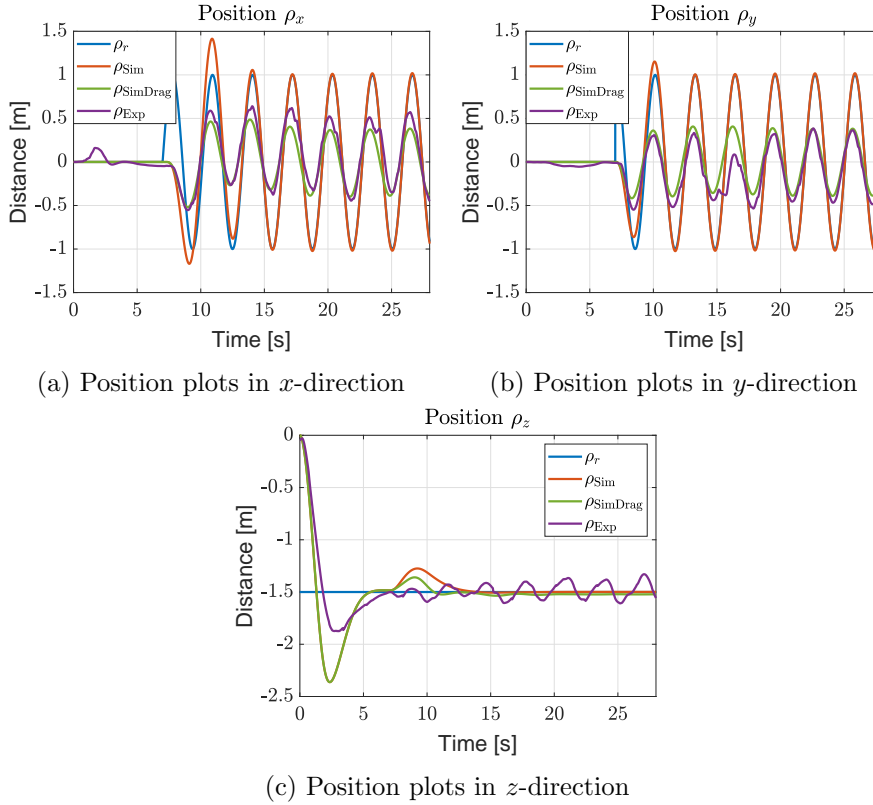
Figure 6.6: Experimental and simulation results of a circular trajectory with and without the drag included in the model, with k_c = 0.22 .
