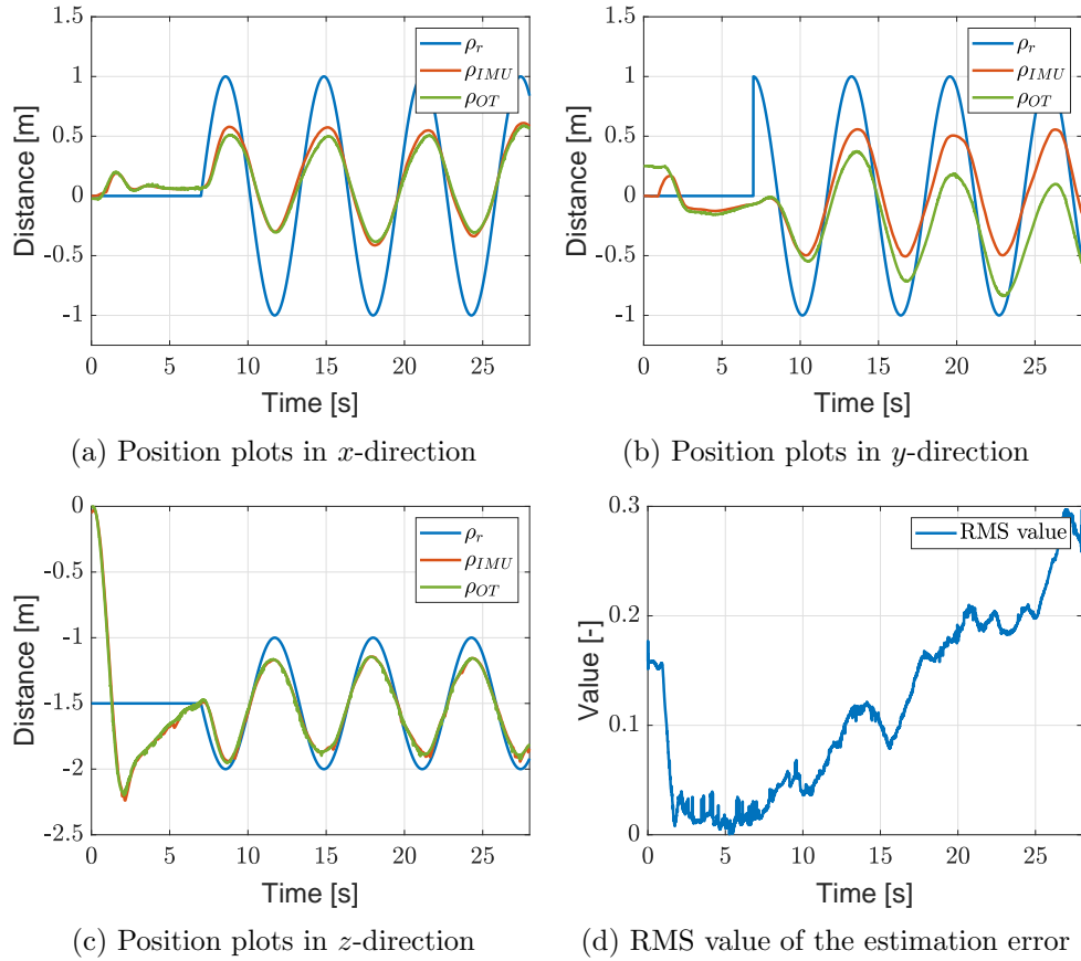
Figure 5.11: Experimental results of a 3D trajectory with the optical flow factor included in the IMU estimator.
