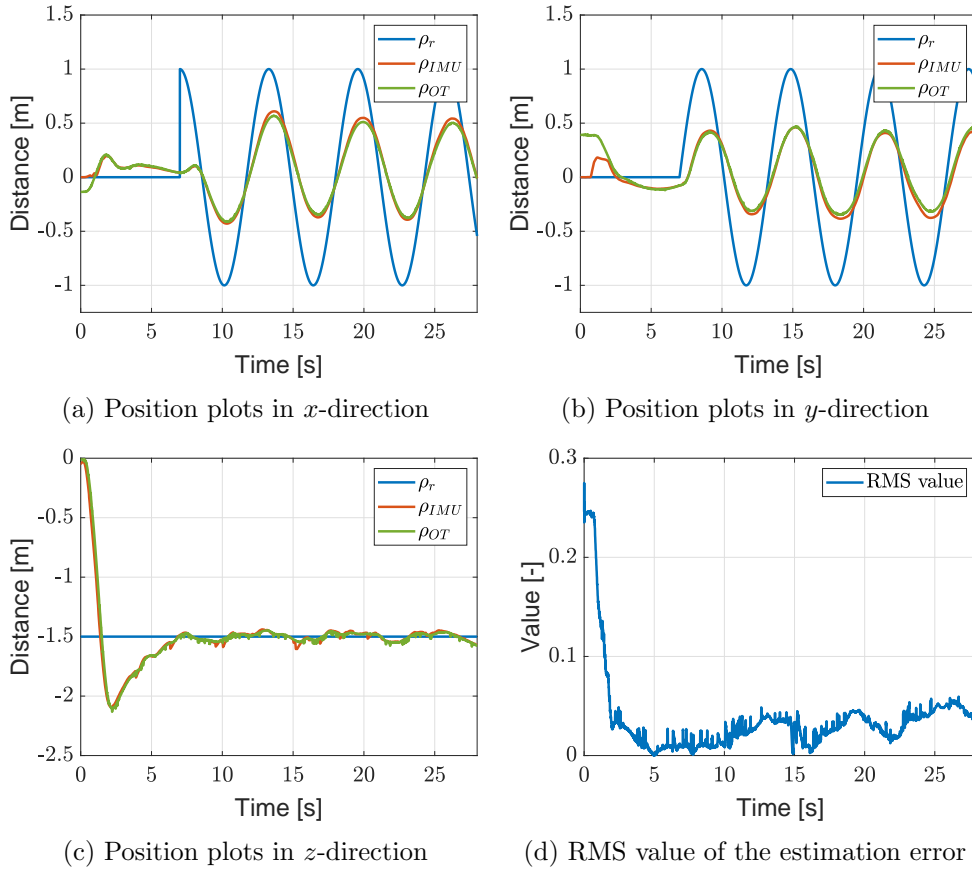
Figure 5.10: Experimental results of a circular trajectory with the optical flow factor included in the IMU estimator.
