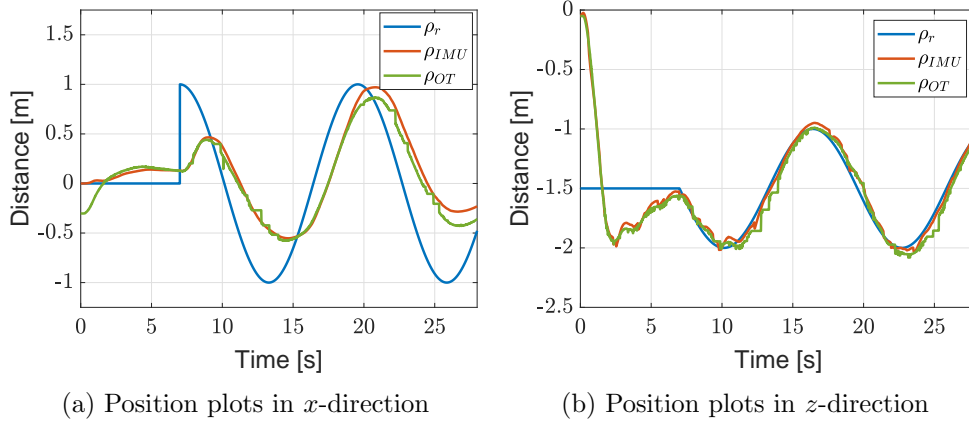
Figure 5.13: Experimental results of a vertical, circular trajectory where a visible drift of the IMU data w.r.t. the Optitrack data in x -direction occurs.
