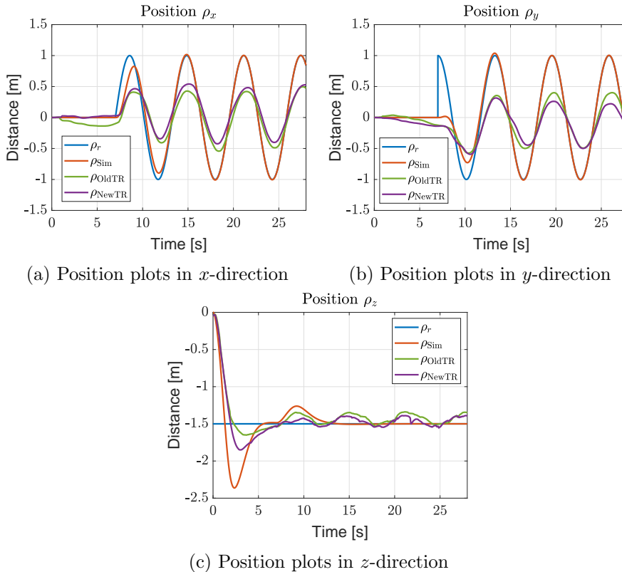
Figure 6.1: Experimental and simulation results of a circular trajectory with both the old and the new thrust ratio.
