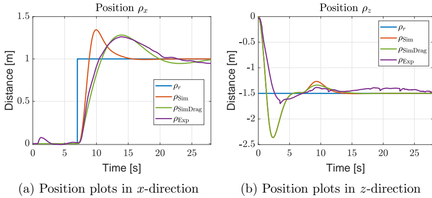
Figure 6.5: Experimental and simulation results of a step response in x direction with and without the drag included in the model, with k_c = 0.22 .
