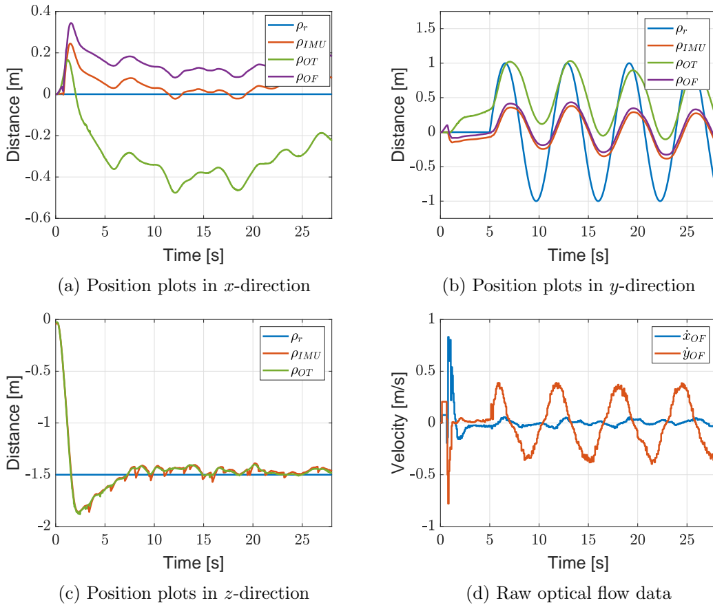
Figure 5.6: Experimental results with the reference signals in blue \rho_r , the estimated values by the default estimator \rho_{IMU} in red, the Optitrack values \rho_{OT} in green and the integrated optical flow \rho_{OF} in purple, except for the raw optical flow data.
