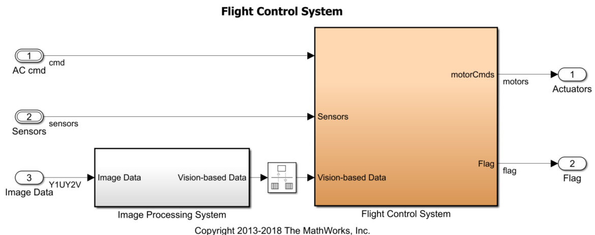
Figure 4.2: The flight control system that is mounted on the drone using the Simulink support package.
