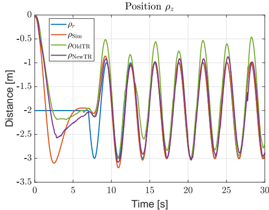
Figure 6.2: Experimental and simulation results of a sine trajectory in z direction.
