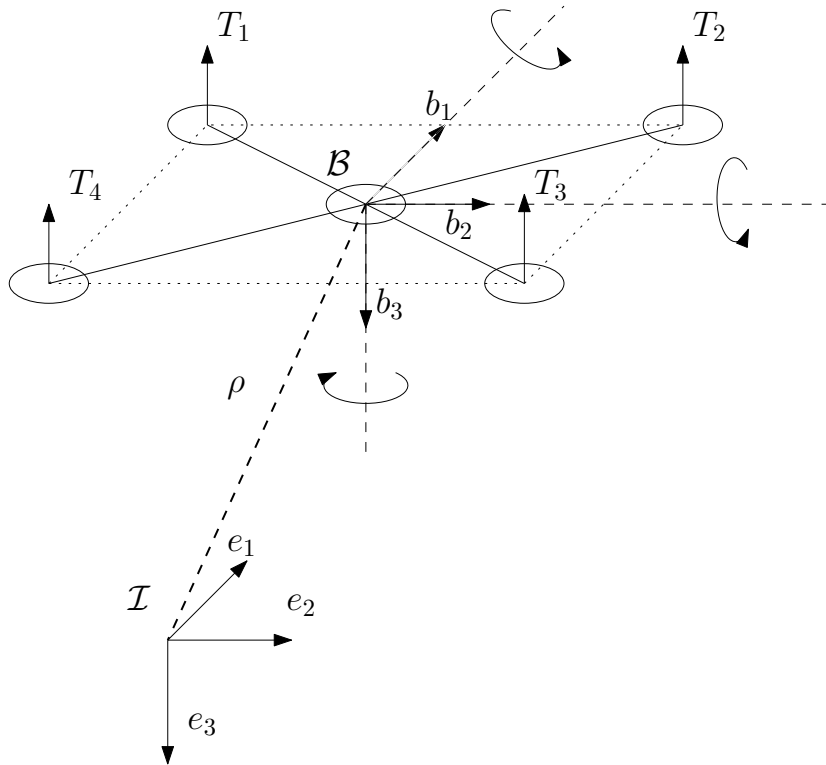
Figure 3.1: Schematic overview of the quadrotor. The inertial frame \mathcal{I} is oriented in a North-East-Down (NED) frame which is fixed to the ground. The body fixed frame \mathcal{B} can be expressed in the inertial frame with a translational component \rho and a rotational component q .
