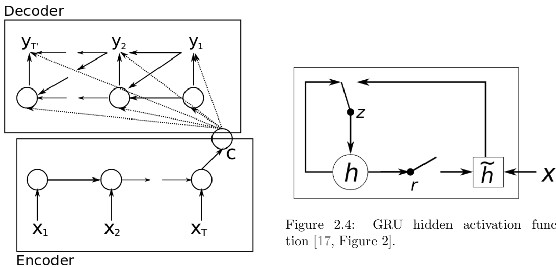
Figure 2.3: RNN Encoder-decoder [17, Figure 1].
