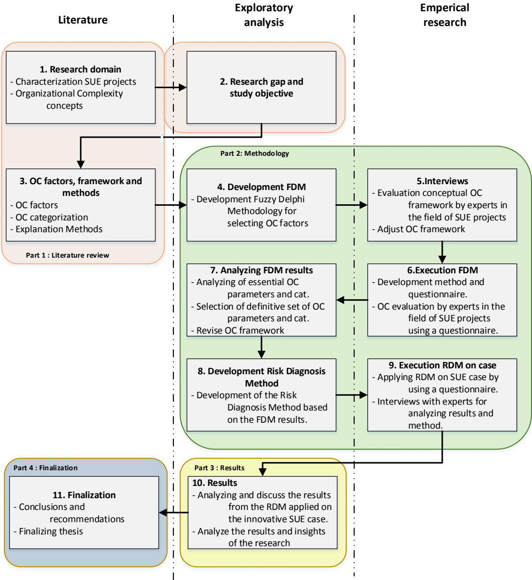
Figure 1-1: Research design.
