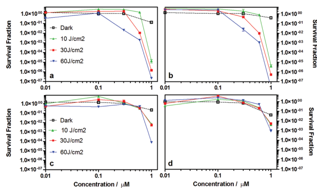
Fig. 4 S. aureus photoinactivation studies with ZnPc (a), ZnPc1 (b), RuPc (c) and RuPc1 (d) upon red light irradiation. Light doses: 10 J cm -2 (triangles), 30 J cm -2 (filled squares), and 60 J cm -2 (inverted triangles). Working concentrations: 0.01, 0.1, 0.3, 0.6 and 1 μM. Dark controls are represented with empty squares. Results are the mean from at least three different experiments.
