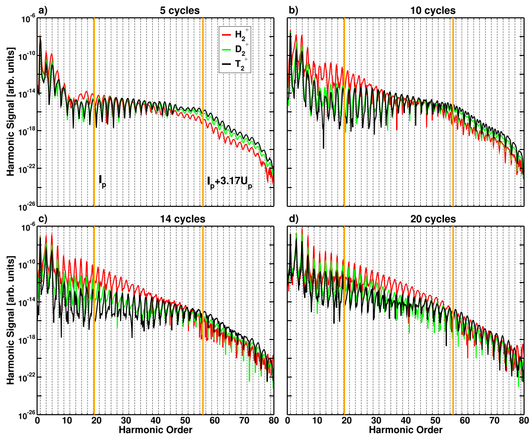
Figure 1. HHG spectrum for a pulse of 800 nm, I = 3 \times 10^{14} W/cm 2 and 5 (a), 10 (b), 14 (c) and 20 (d) optical cycles for H_2^+ , D_2^+ and T_2^+ . The dashed vertical lines indicate odd harmonics. The thick vertical lines indicate the ionization threshold (left line) and the cut-off energy obtained from E_{\text{cutoff}} = I_p + 3.17U_p (right line).
