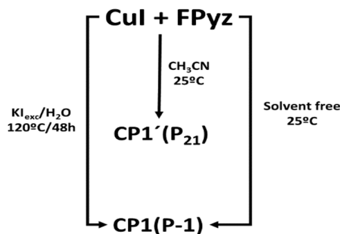
Scheme 1. Synthetic Routes to get CP1 and CP1' Polymorphs (2-Fluoropyrazine (FPyz))
