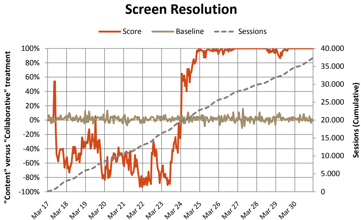
Figure 35: Score and baseline for the "Screen Resolution" context
