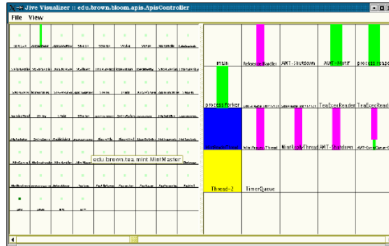
Figure 5.4: A typical view of Jive, from [19]. On the left, the class and package view. On the right, the thread view.
