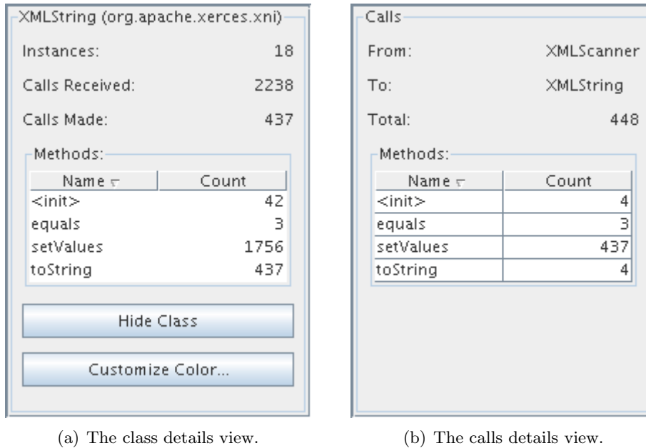
Figure 4.11: Detail views.
