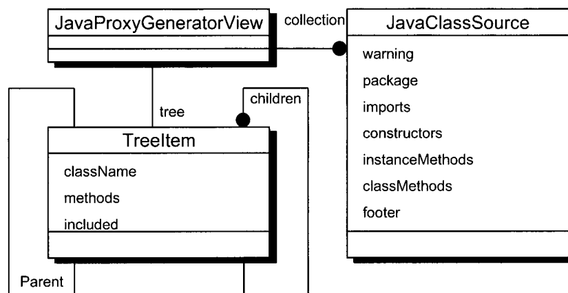
Figuur 32 Attributen in de Javaproxygenerator
