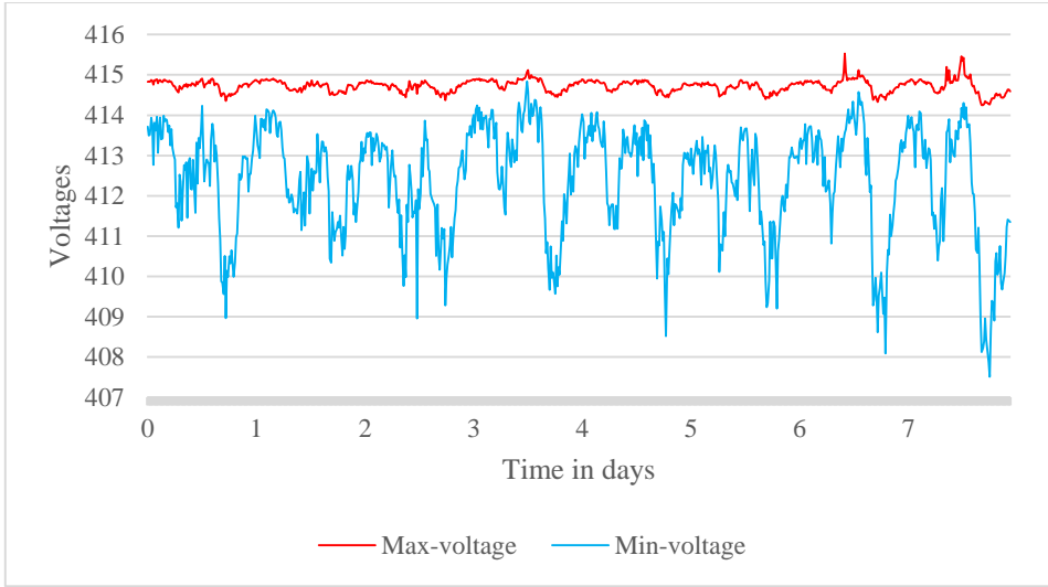
FIGURE 12: VOLTAGES IN GRID IN WINTER SCENARIO OVER THE LENGTH OF THE WINTER DATASET
