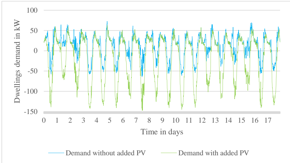
FIGURE 13: POWER SUPPLIED TO NEIGHBOURHOOD IN SUMMER SCENARIO IN kW OVER THE LENGTH OF THE DATASET
