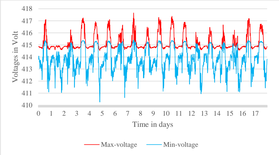
FIGURE 11: VOLTAGES IN GRID IN SUMMER SCENARIO OVER THE LENGTH OF THE SUMMER DATASET
