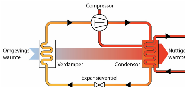
Figure 6.4 Schematic diagram of a heat pump.
