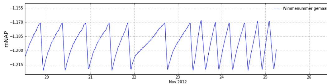
Figure 3.10 water level controlled by a pumping station. Source: http://hknk.lizard.net/map/workspace/peilstanden/
