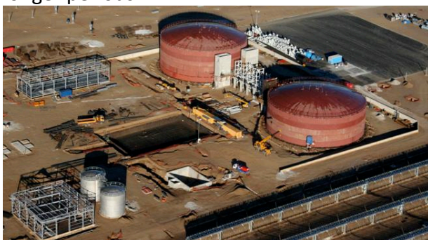
Figure 3.2 Heat storage tanks in can be used to increase the flexibility in a demand management application related to thermal applications
