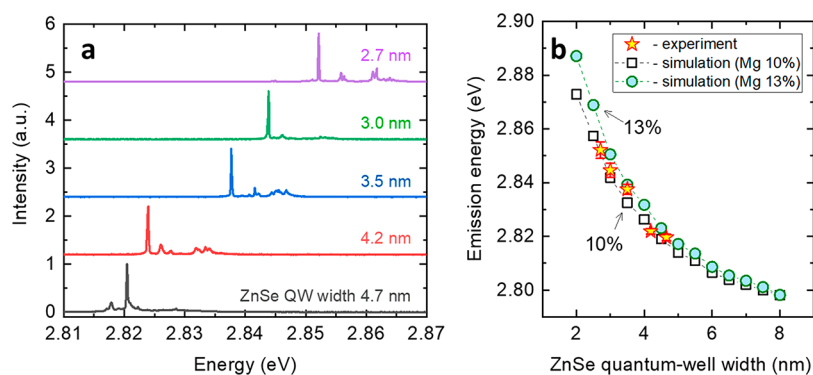
Figure 3. Coarse-tuning of single-photon emission. (a) Typical PL spectra measured for the NPs with different ZnSe QW widths under the same experimental conditions. The shift of the D^0X emission peak reflects the wavelength coarse-tuning of our developed NPs. (b) PL emission energy of the donor-bound-exciton as a function of ZnSe QW width obtained for experimental and simulated data. The simulations were performed for ZnMgSe/ZnSe/ZnMgSe QW stacks with 10% and 13% Mg concentration, respectively, as typical Mg contents in the ZnMgSe barriers of the measured samples. Vertical error bars in the experimental data represent the standard deviation of the mean values calculated for each set of studied NPs with different QW widths.
