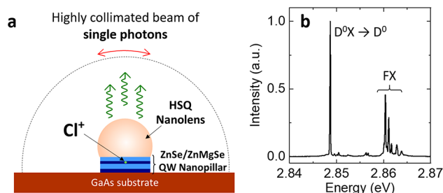
Figure 1. (a) Schematic illustration of a Cl-doped ZnSe/ZnMgSe QW NP with spherical-shaped HSQ nanolens on top that helps to collect the emitted photons. (b) Typical PL spectrum measured for a ZnSe/ZnMgSe NP (ZnSe QW width of approximately 2.71 nm) with a spherical-shaped lens at a temperature of 5 K and with 5 \mu W pulsed laser excitation. The spectrum reveals a single-photon emission line at 2.848 eV that originates from the recombination of donor-bound excitons ( D^0X \rightarrow D^0 ). The FX-labeled group of peaks corresponds to the recombination of heavy-hole free excitons.
