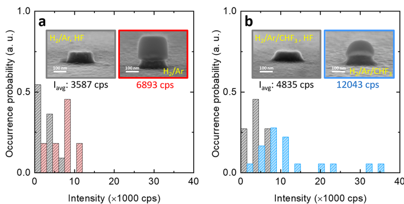
Figure 4. Histograms of the PL intensity distributions measured for the D^0X emission from NPs with and without HSQ lenses etched using (a) H_2/Ar or (b) H_2/Ar/CHF_3 RIE plasma. The histogram bin-width of 3000 cps is used. The mean average values of each intensity distribution are indicated under the corresponding SEM insets, which represent a typical NP for each set of measured devices. For the NPs covered with spherical-shaped HSQ nanolenses and etched using H_2/Ar/CHF_3 RIE plasma (shown in blue), we observe up to 1 order of magnitude increase in the external quantum efficiency.
