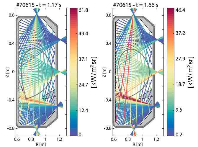
Fig. 4. Bolometry line of sight intensity before and after creation of XPR in TCX #70615. The peak of radiation moves from outside (left) to inside the confined region (right). (For interpretation of the references to colour in this figure legend, the reader is referred to the web version of this article.)
