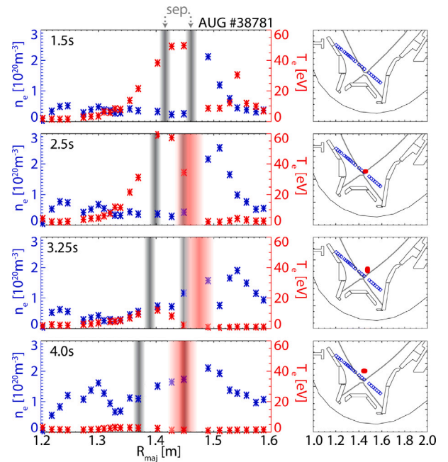
Fig. 2. T_e and n_e from DTS at different time points in AUG #38781. The grey shaded areas indicate intersection of the DTS beam path with the separatrix, the red shaded area the radial location and width of the XPR (note: the XPR might be vertically higher than the DTS measurement location, thus, these measurements are located between the XPR and the separatrix). Right: Location and extend (FWHM) of the XPR (red) and the location of the DTS measurements (blue). (For interpretation of the references to colour in this figure legend, the reader is referred to the web version of this article.)
