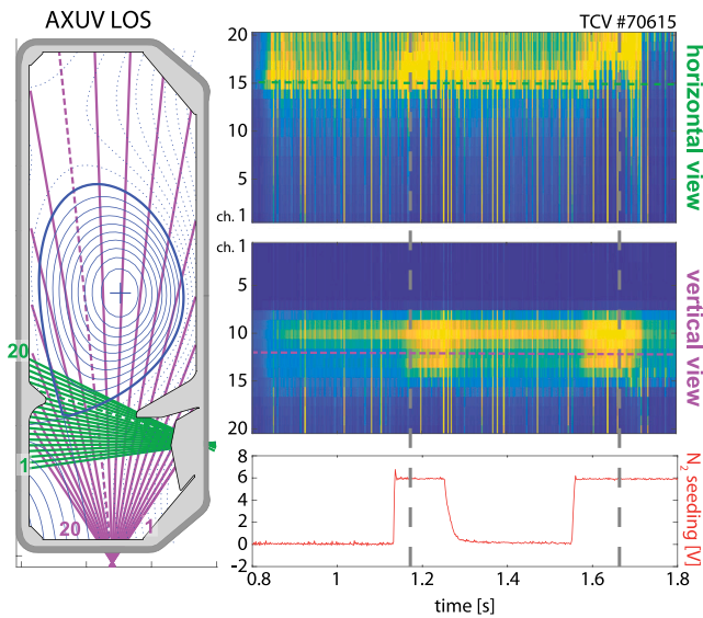
Fig. 3. Left: LOS location of AXUV channels. Right: Contour plot of the measured intensity of the AXUV cameras from the side (top) and from below (middle), showing the shift of radiation depending on the nitrogen seeding rate (bottom). The most significant LOS are indicated by the dashed lines, the vertical grey lines indicate time points shown in Fig. 4. (For interpretation of the references to colour in this figure legend, the reader is referred to the web version of this article.)
