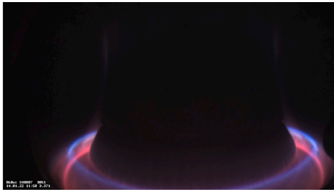
Fig. 1. Visible camera image of a discharge with an XPR (AUG #40007, 3.4 s) seen in blue light emitted by nitrogen, dominated by N^{2+} . Magenta is the typical Balmer emission from deuterium in a divertor leg. (For interpretation of the references to colour in this figure legend, the reader is referred to the web version of this article.)
