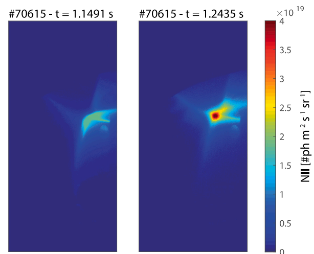
Fig. 5. Filtered camera image of an NII spectral line (399.0 nm) by MANTIS before (left) and after (right) development of XPR in TCX #70615. (For interpretation of the references to colour in this figure legend, the reader is referred to the web version of this article.)
