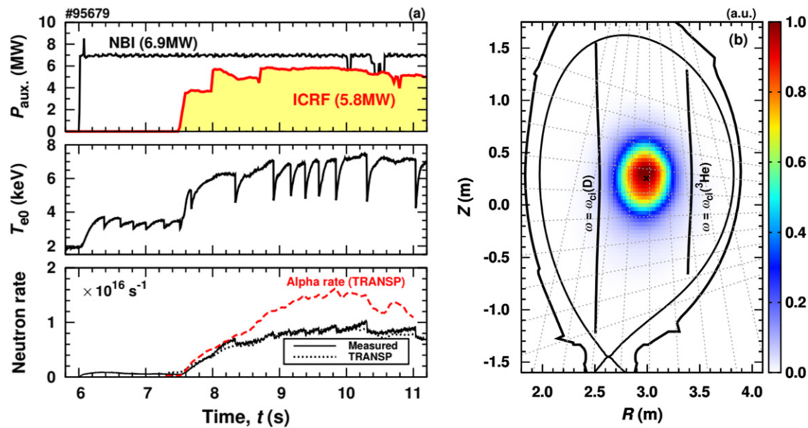
Figure 3. (a) Pulse #95679, with the three-ion D–( \text{D}_{\text{NBI}} )– ^3\text{He} scenario applied for heating and FI generation. The bottom panel shows the simulated (TRANSP) D–D neutron and D– ^3\text{He} \alpha rates. (b) Spatial profile of D–D neutron emission. Figure reproduced from [29].
