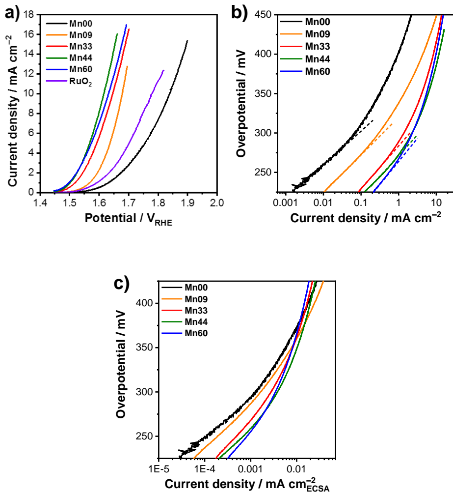
Figure 3.4. a) Linear sweep voltammograms and b) corresponding Tafel plots of the anodes recorded in 0.1 M H 2 SO 4 . Linear Tafel regions are indicated by dashed lines. c) Tafel plots of the electrodes normalized with ECSA.
