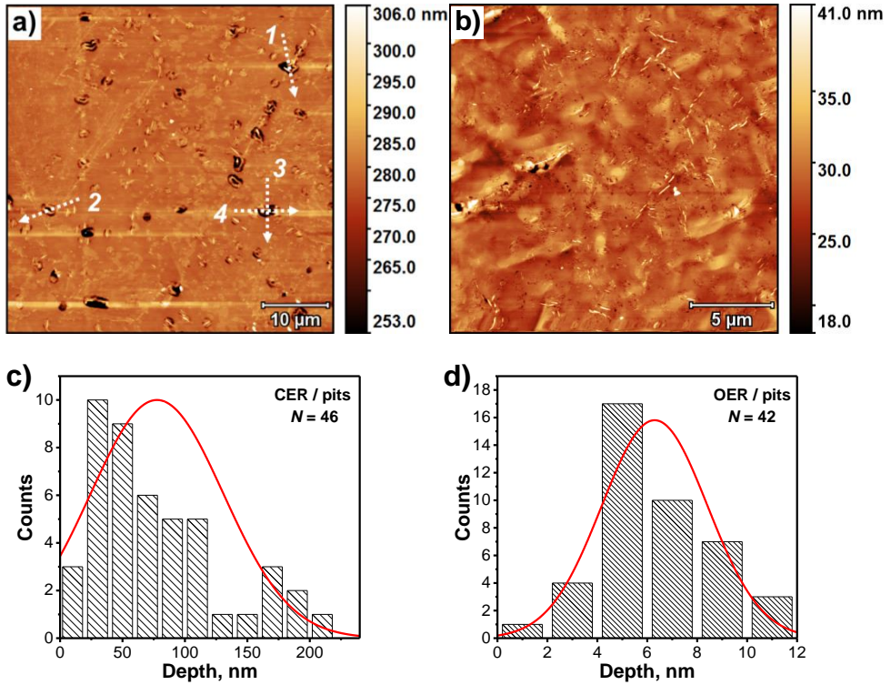
Figure A8. AF micrographs of spent \text{RuO}_2(110)/\text{Ru}(0001) subjected to a) CER and b) OER treatments; c, d) corresponding histograms of depth distribution of pits.
