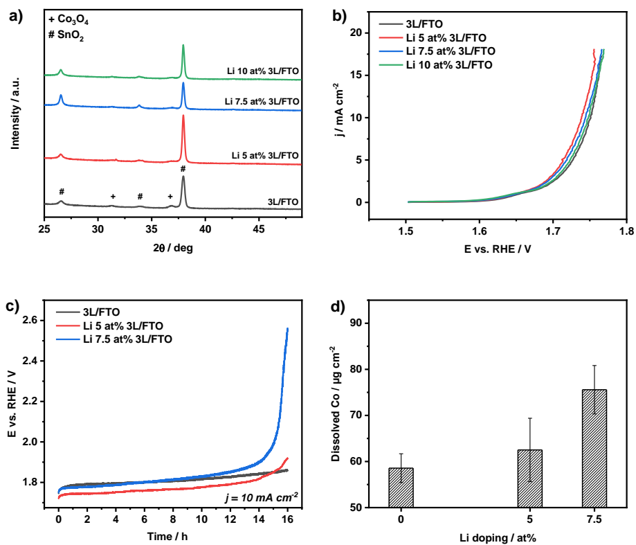
Figure 6.7. Effect of Li doping on the structure and acidic OER activity and stability of 3L/FTO sample: a) XRD; b) Linear Sweep Voltammetry; c) Chronopotentiometry; d) Chronopotentiometry conducted at j = 10 \text{ mA cm}^{-2} ; amount of leached Co in the electrolyte during the chronopotentiometry measured by ICP-OES.
