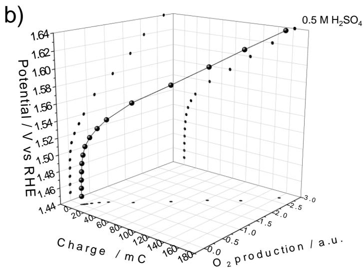
Figure A2. Three-dimensional representations of the results of OLEMS experiments conducted in a) 0.5 M HCl and b) 0.5 M H 2 SO 4 , which report the gas production versus the applied potential and charge.
