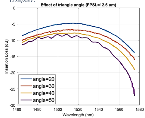
Figure 5. Effect of triangle angle on the transmitted power of the grating couplers, FPSL=12.6 \mu\text{m} .
