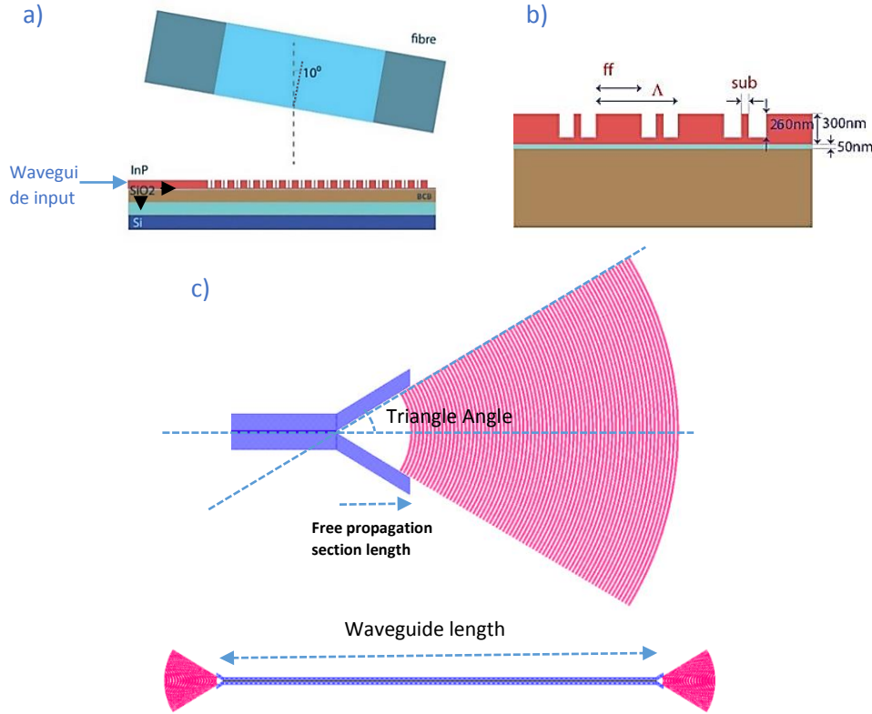
Figure 1. (a) Schematic illustration of the position of the grating with respect to the optical fiber, (b) simulation parameters for optimization. (c) Schematic illustration of the design and related parameters.
