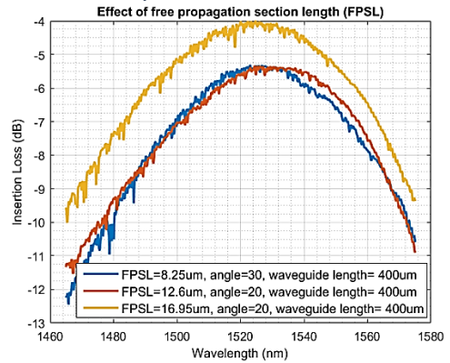
Figure 6. Effect of free propagation section length, comparison between highest transmitted powers for each FPSL.
