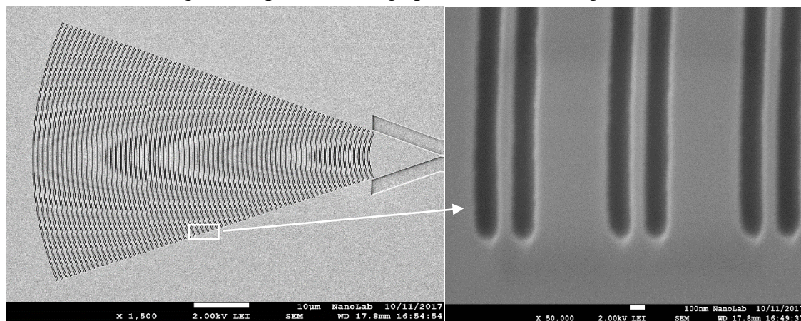
Figure 3. (a) SEM image of the fabricated grating coupler, (b) magnified inset of the grating lines.
