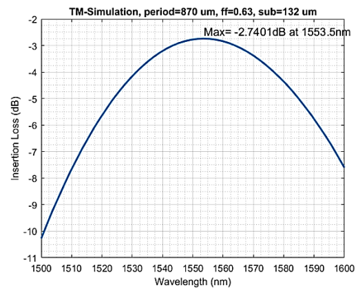
Figure 2. Simulation results for focusing subwavelength TM grating coupler.
