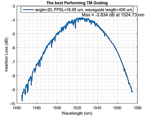
Figure 4. The best performing grating coupler.
