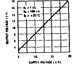
LH0033 Output Voltage vs Supply Voltage
