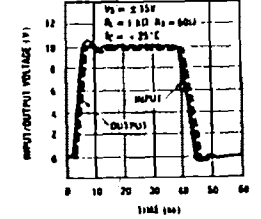
LH0033 Positive Pulse Response
