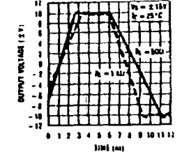
LH0063 Large Signal Pulse Response
