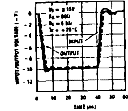
LH0033 Negative Pulse Response
