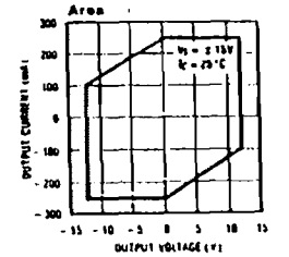
LH0063 DC Safe Operating Area
