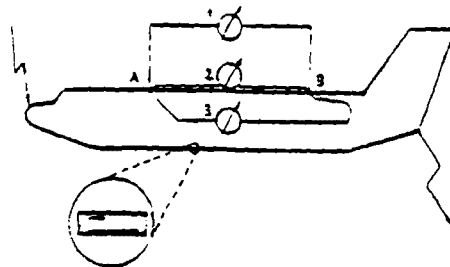
Fig. 3: The voltage between the points A and B of an airplane, caused by lightning current, cannot be described by a potential difference; each of the three voltmeters gives a different reading, depending on the loop enclosed by the leads.
