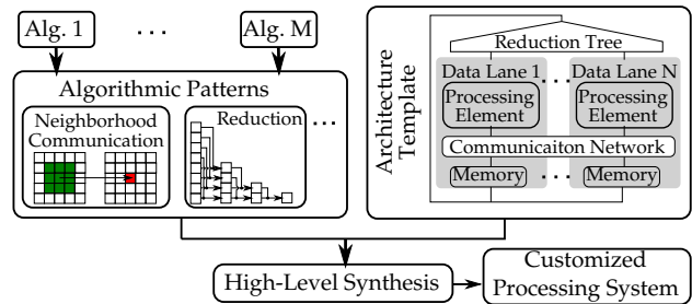
Fig. 4. High-level synthesis based on algorithmic patterns and architecture templates.
