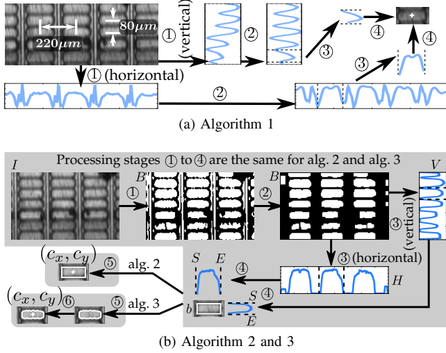
Fig. 7. Illustration of each processing stage of three vision algorithms.
