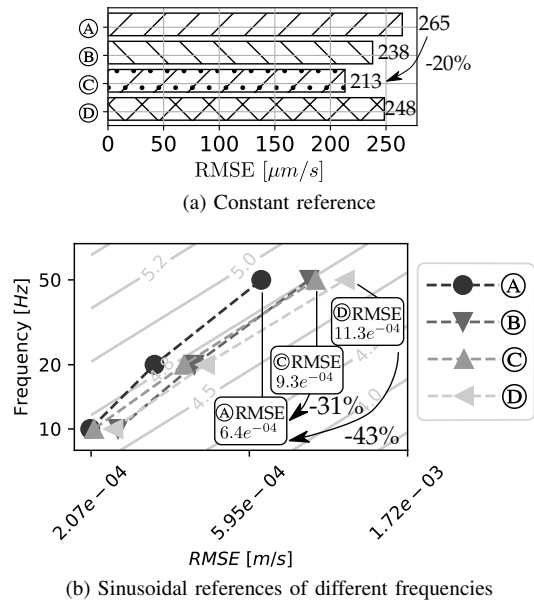
Fig. 15. RMSE of tracking: (a) a constant reference described in (8); (b) sinusoidal references of different frequencies f described in (9). In (b), besides four configurations \textcircled{A} - \textcircled{D} , equal- (f/RMSE) lines are plotted, with the values of \log(f/RMSE) annotated along the lines.
