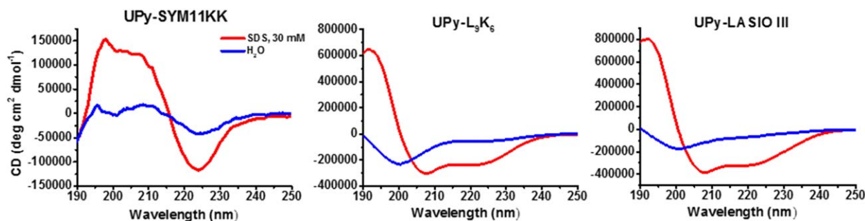
FIGURE 2 Folding of the UPy-antimicrobial peptides. CD spectra of UPy-AMPs (50 \mu M) in water ( \text{H}_2\text{O} ; blue line) or 30 mM sodium dodecyl sulfate (SDS; red line) at 25 ^\circ\text{C} . [Color figure can be viewed at wileyonlinelibrary.com ]
