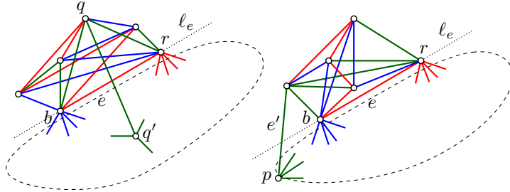
Figure 3: Two examples depicting the construction of three edge-disjoint plane spanning trees on S .
