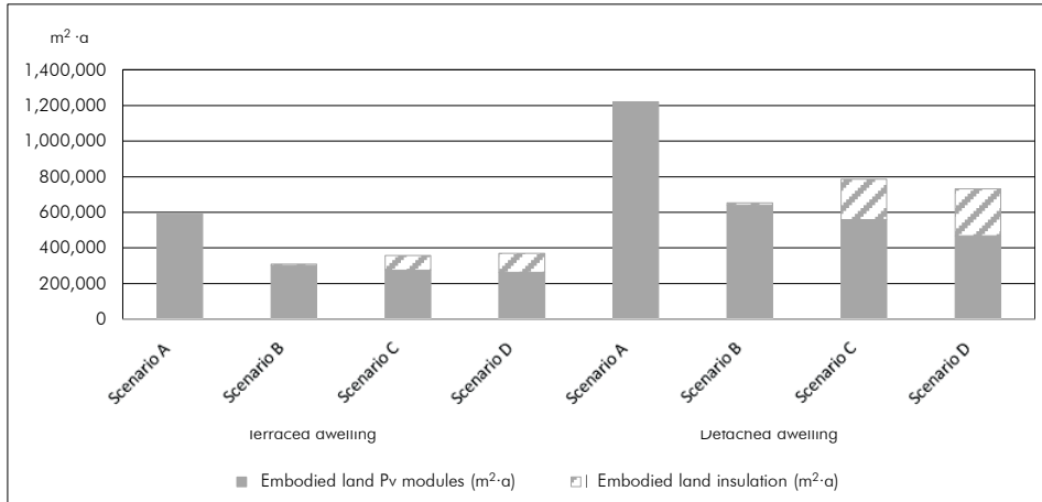
Figure 12. Embodied land (m 2 ·a) of the different scenarios in the two dwelling types.
