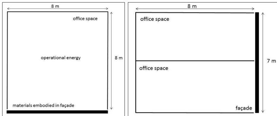
Figure 5 and 6. Floor plan and section of the investigated simulated south facing office space.
