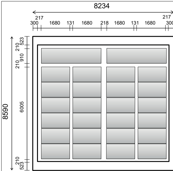
Figure 4. Top view of the BIPV rooftop design with 24 PV modules under investigation in this study (sizes in mm). Two solar thermal collectors, indicated above the 24 PV modules, are not included in this research.
