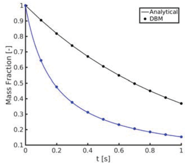
Figure 2: First (top line) and second (bottom line) order reactions in a batch reactor: comparison with the analytical solutions.
