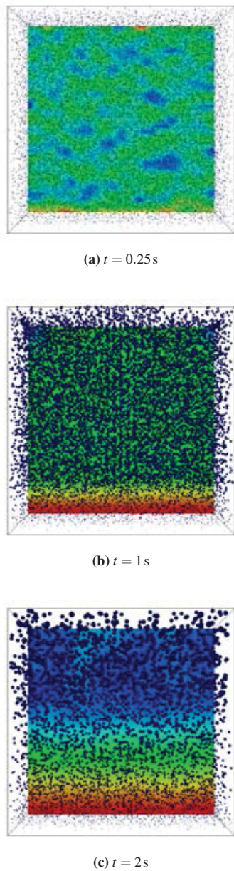
Figure 4: Snapshots of the concentration profiles around bubbles for the bulk nucleation case. The color range from higher dissolved gas concentration (red) to lower (blue).
