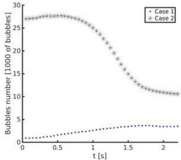
Figure 6: Comparison of the bubble density in the column for the two cases: Case 1 nucleation on a surface and Case 2 in the liquid bulk.
