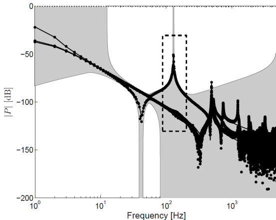
Figure 1: Bode magnitude diagram: nonparametric estimate (dot), nominal model (black) and model set (dashed).
