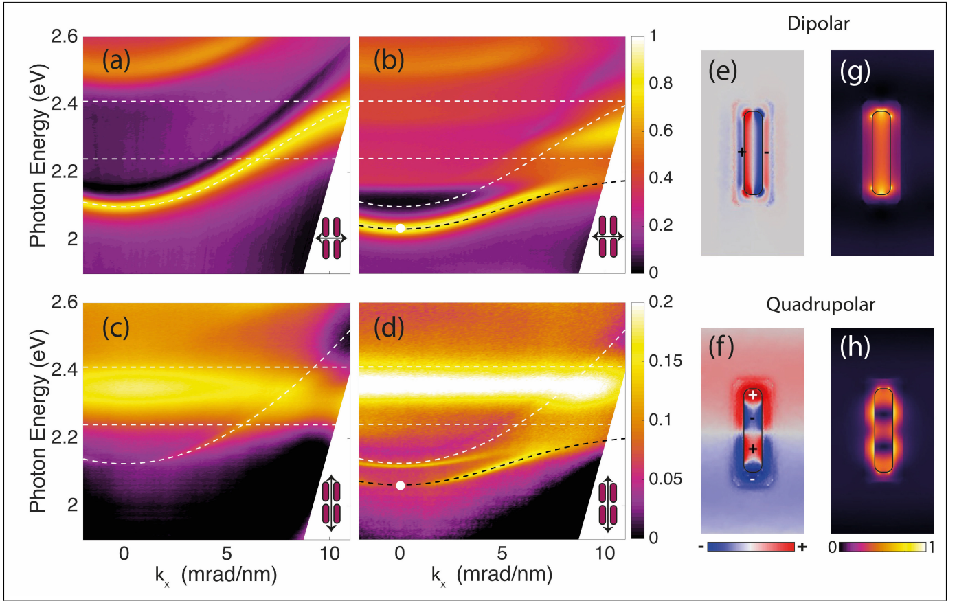
FIG. 2. The extinction measurements of the sample with incident light polarized along the short axis of the nanoparticles in the absence (a) and the presence (b) of the dye molecules. The extinction of the same sample illuminated by the light polarized along the long axis of the nanoparticles without (c) and with (d) the dye. The white dashed lines indicate the energies of the two strongest vibronic transitions in the molecules (horizontal lines) and the SLR dispersion whereas the dashed black lines correspond to PEP modes. Maps of the induced charge density (e,f) and normalized electric field amplitude (g,h) for the corresponding lowest PEP modes at k_x = 0 mrad/nm. (e,g) correspond to the bright (dipolar-like) resonance, while (f,g) to the dark (quadrupolar) resonance at k_x = 0 mrad/nm.
