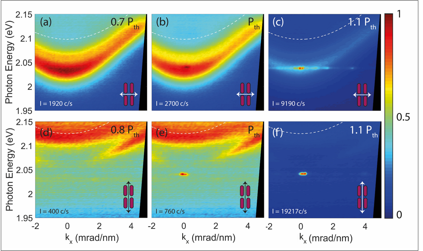
FIG. 4. Normalized angular-resolved emission measurements for two detection polarizations, parallel and orthogonal to the long axis of the nanoparticles, for the array of nanoparticles covered with PMMA with the dye concentration of 35 wt %. The cartoon in the inset of each panel depicts the orientation of the nanoparticles with an arrow indicating the direction of the transmission axis of the polarization analyzer. The emission intensity in unit of counts/s at E = 2.04 eV and k_x = 0 mrad/nm for each detection condition is indicated at the bottom of each panel. (a-c) Angle-resolved PL for different pump fluences with the analyzer along the short axis of the nanoparticle visualizing to the bright mode along (0, \pm 1) RAs supported by the array. (d-f) Angle-resolved PL for different pump fluences with analyzer along the long axis of the nanoparticle. In this configuration, the dark mode excited by (0, \pm 1) RAs is probed. The bare modes associated with the uncoupled SLRs are shown by white dashed line in each panel.
