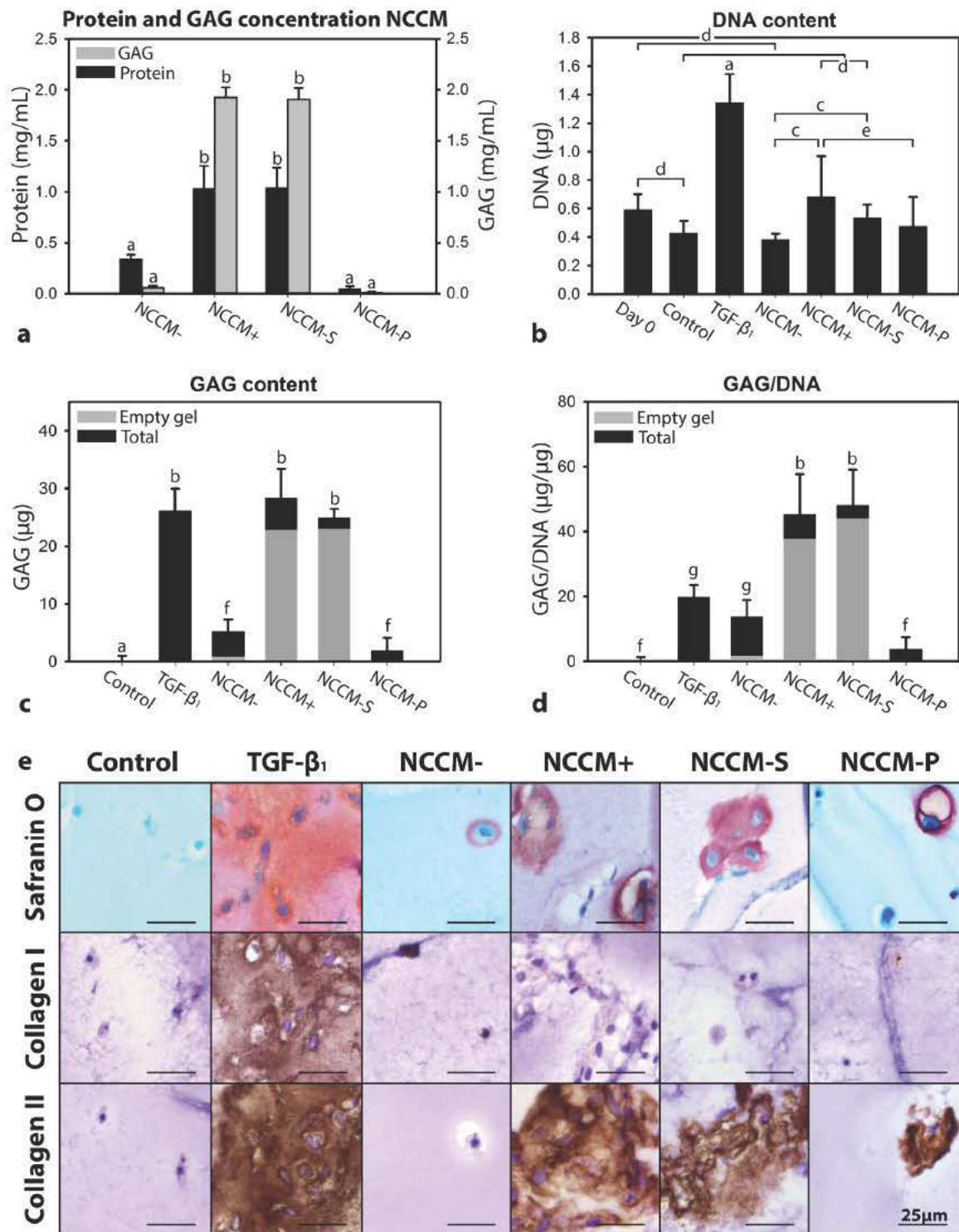
Fig. 3. Both soluble and pelletable factors derived from canine NC-conditioned medium (NCCM) exert anabolic effects on canine chondrocyte-like cells (CLCs) derived from degenerated intervertebral discs (IVDs). Cell proliferation and matrix production of canine CLCs cultured in hydrogels in basal culture medium (control), basal culture medium supplemented with 10 ng/mL TGF- \beta_1 , NCCM from dedifferentiated NCs (NCCM-), NCCM from healthy NCs (NCCM+), and the soluble (NCCM-S) and pelletable (NCCM-P) fraction of NCCM+, which were separated by ultracentrifugation. (a) Protein (black) and glycosaminoglycan (GAG, grey) concentration (mean \pm SD) of canine NCCM (fractions). (b-d) DNA, GAG and GAG/DNA content (mean \pm SD) of canine CLC hydrogels at day 28. The grey colour in the black bars indicates the level of GAGs present in cell-free NCCM-treated hydrogels for these conditions. (e) Safranin O/Fast Green staining and collagen type I and II immunohistochemistry of canine CLC hydrogels at day 28. Significant differences are indicated for non-corrected data (not corrected for empty gels). a, significant difference between this condition and all other conditions ( p < 0.001 ); b, significant difference between this condition and all other conditions except for the other condition indicated with 'b' ( p < 0.001 ); c, d and e, significant difference between these conditions with p < 0.001 , p < 0.01 and p < 0.05 , respectively; f and g, significant difference between this condition and all other conditions with p < 0.01 and p < 0.05 , respectively; n = 8 for DNA and GAG content and n = 4-8 for histology.
