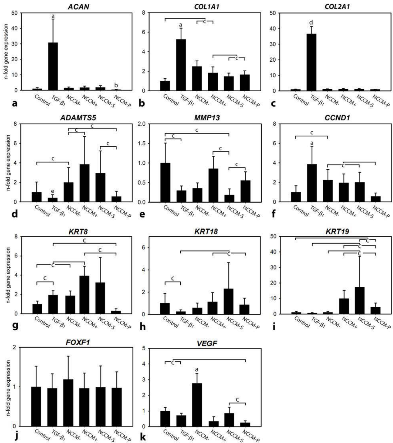
Fig. 4. Only the soluble factors present in canine NC-conditioned medium (NCCM) stimulate expression of genes related to cell proliferation of canine chondrocyte-like cell (CLC), but none of the NCCM (fractions) effects expression of genes related to matrix production. Target gene expression levels of canine CLCs cultured in hydrogels in basal culture medium (control), basal culture medium supplemented with 10 ng/mL TGF-β 1 , NCCM from dedifferentiated NCs (NCCM-), NCCM from healthy NCs (NCCM+), and the soluble (NCCM-S) and pelletable (NCCM-P) fraction of NCCM+, which were separated by ultracentrifugation. (a-k) Relative ACAN , COL1A1 , COL2A1 , ADAMTS5 , MMP13 , CCND1 , KRT8 , KRT18 , KRT19 , FOXF1 , and VEGF gene expression (mean ± SD) of the hydrogels at day 4. The control hydrogels were set at 1. a, significant difference between this condition and all other conditions ( p < 0.05 ); b, significant difference between this condition and all other conditions except control ( p < 0.05 ); c, significant difference between these conditions ( p < 0.05 ); d, significant difference between this condition and all other conditions ( p < 0.01 ); e, significant difference between this condition and all other conditions except NCCM-P ( p < 0.05 ); n = 8 .
