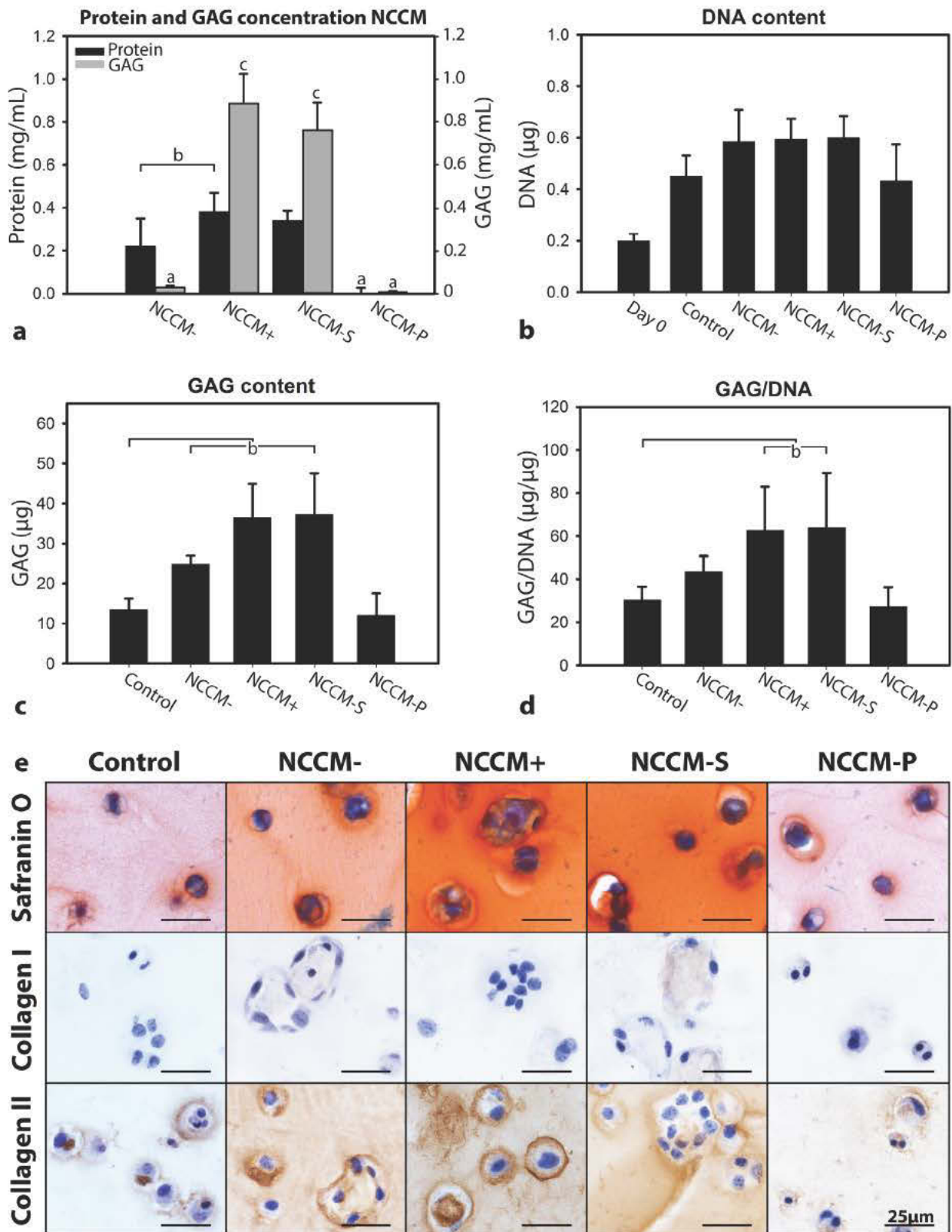
Fig. 2. Soluble factors derived from porcine NC-conditioned medium (NCCM) exert anabolic effects on bovine chondrocyte-like cells (CLCs) derived from caudal intervertebral discs (IVDs). Cell proliferation and matrix production of bovine CLCs cultured in alginate beads in basal culture medium (control), NCCM from dedifferentiated NCs (NCCM-), NCCM from healthy NCs (NCCM+), and the soluble (NCCM-S) and pelletable (NCCM-P) fraction of NCCM+, which were separated by ultracentrifugation. (a) Protein (black) and glycosaminoglycan (GAG, grey) concentration (mean \pm SD) of porcine NCCM (fractions). (b-d) DNA, GAG and GAG/DNA content (mean \pm SD) of bovine CLC alginate beads at day 28. (e) Safranin O/Fast Green staining and collagen type I and II immunohistochemistry of bovine CLC alginate beads at day 28. a, significant difference between this condition and all other conditions ( p < 0.05 ); b, significant difference between these conditions ( p < 0.05 ); c, significant difference between this condition and all other conditions except for the other condition indicated with 'c' ( p < 0.05 ); n = 4 .
