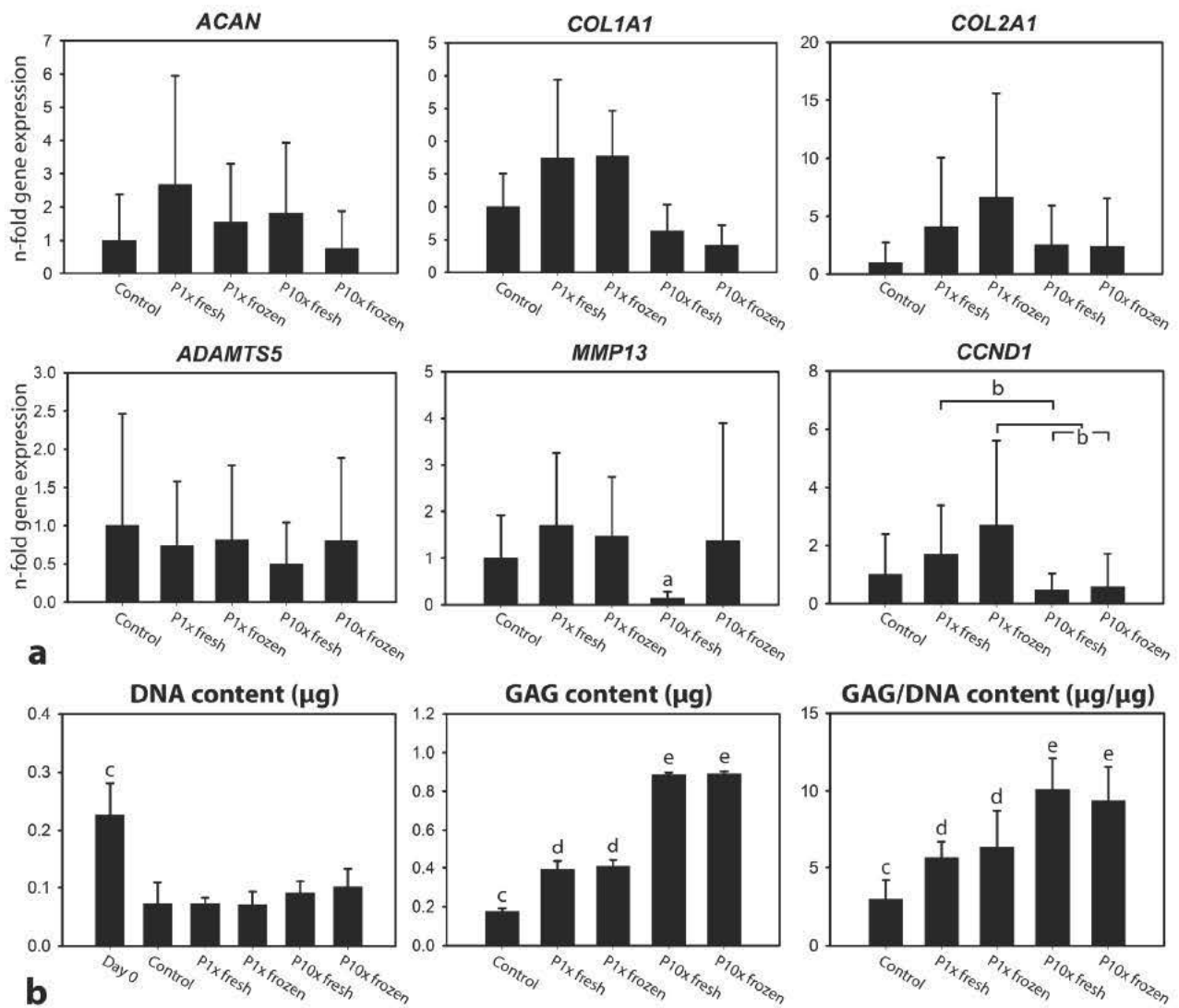
Fig. 5. Frozen canine pelletable NCCM factors exert comparable anabolic effects as freshly applied (non-frozen) pelletable NCCM factors, while a ten times higher concentration of pelletable factors induces a more pronounced effect on canine chondrocyte-like cell (CLC) matrix production. Target gene expression levels and DNA and glycosaminoglycan (GAG) content of canine CLCs cultured in micro-aggregates in basal culture medium (control), or 1× concentrated freshly generated, non-frozen NCCM-P (P1× fresh), 1× concentrated NCCM-P frozen at -70 °C (P1× frozen), 10× concentrated freshly generated, non-frozen NCCM-P (P10× fresh) and 10× concentrated frozen NCCM-P (P10× frozen). (a) Relative ACAN , COL1A1 , COL2A1 , ADAMTS5 , MMP13 and CCND1 gene expression (mean ± SD) of the micro-aggregates at day 4. The control micro-aggregates were set at 1. (b) DNA, GAG and GAG/DNA content (mean ± SD) of the canine CLC micro-aggregates at day 7. a, significant difference between this condition and all other conditions ( p < 0.05 ); b, significant difference between these conditions ( p < 0.05 ); c, significant difference between this condition and all other conditions ( p < 0.01 ); d, significant difference between this condition and all other conditions except for the other condition indicated with 'd' ( p < 0.01 ); e, significant difference between this condition and all other conditions except for the other condition indicated with 'e' ( p < 0.01 ); n = 8 .
