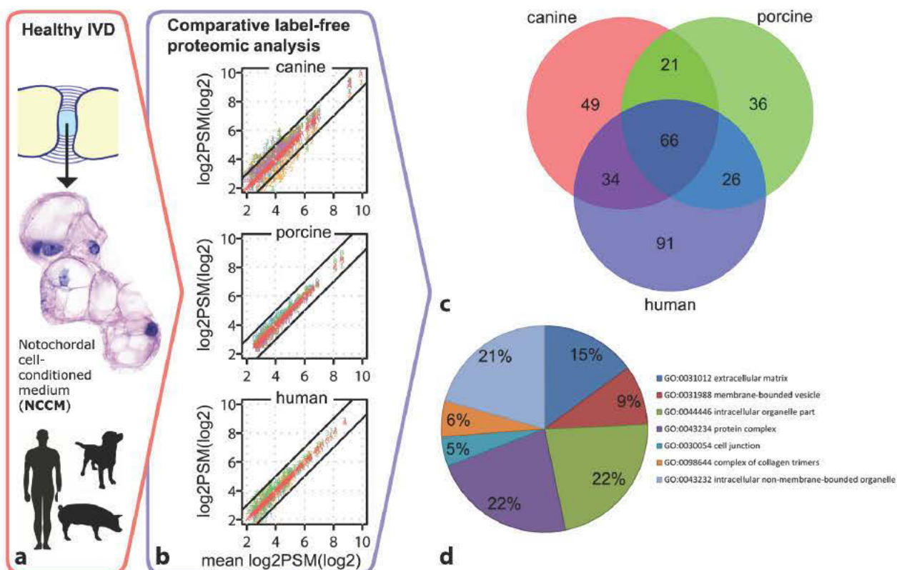
Fig. 1. Proteomic analysis of porcine, canine and human notochordal cell (NC)-conditioned medium (NCCM). (a) NCCM was generated from NC-rich nucleus pulposus (NP) tissue of porcine ( n = 5 ), canine ( n = 5 ) and human ( n = 3 ) donors. (b) Log 2 values of the number of peptide spectrum matches (PSM) plotted against the average number of PSMs for each protein show a higher inter-donor variability for canine NCCM than for porcine and human NCCM. (c) The number of proteins discovered in porcine, canine and human NCCM, and their combinations. (d) Cell and/or matrix origins of the 66 proteins in common to all three species NCCM.
