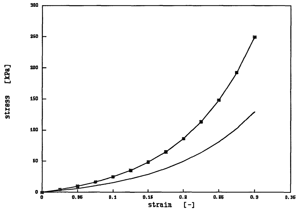
FIGURE 3: Stress versus strain curves in fiber and cross-fiber direction of the endocardial layers are shown. The curve with symbol is svs-curve in ff-direction.
